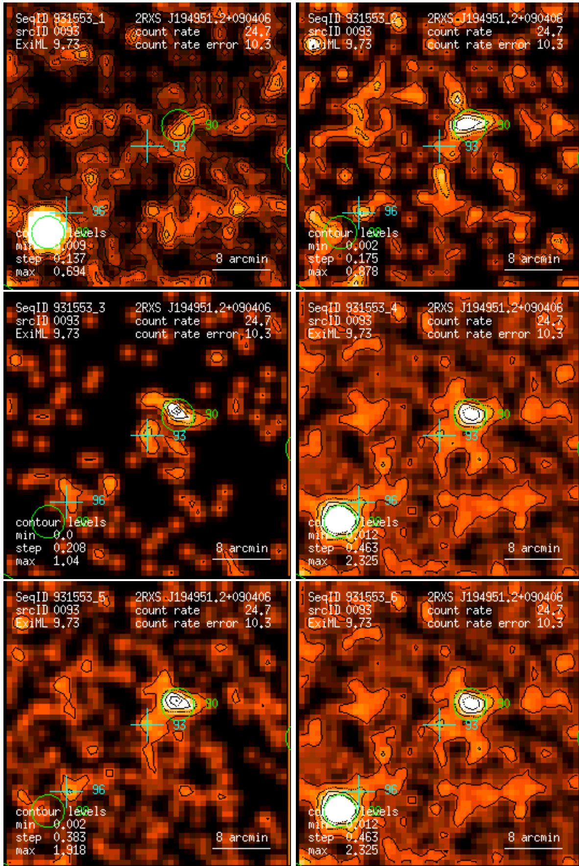
Figure 93: RASS 931553: detection 0093: band rate images, Gaussian filter: (1) PSPC channels 11 – 41, (2) 52 – 90, (3) 91 – 201, (4) 11 – 235, (5) 52 – 201, (6) 11 – 201. Broad band rates in counts/ks. Band rate contour levels in counts/ks/arcmin 2 .
