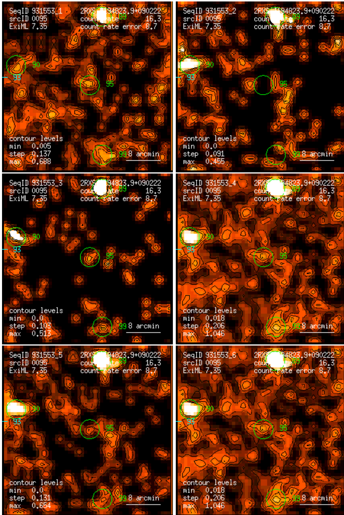
Figure 95: RASS 931553: detection 0095: band rate images, Gaussian filter: (1) PSPC channels 11 – 41, (2) 52 – 90, (3) 91 – 201, (4) 11 – 235, (5) 52 – 201, (6) 11 – 201. Broad band rates in counts/ks. Band rate contour levels in counts/ks/arcmin 2 .
