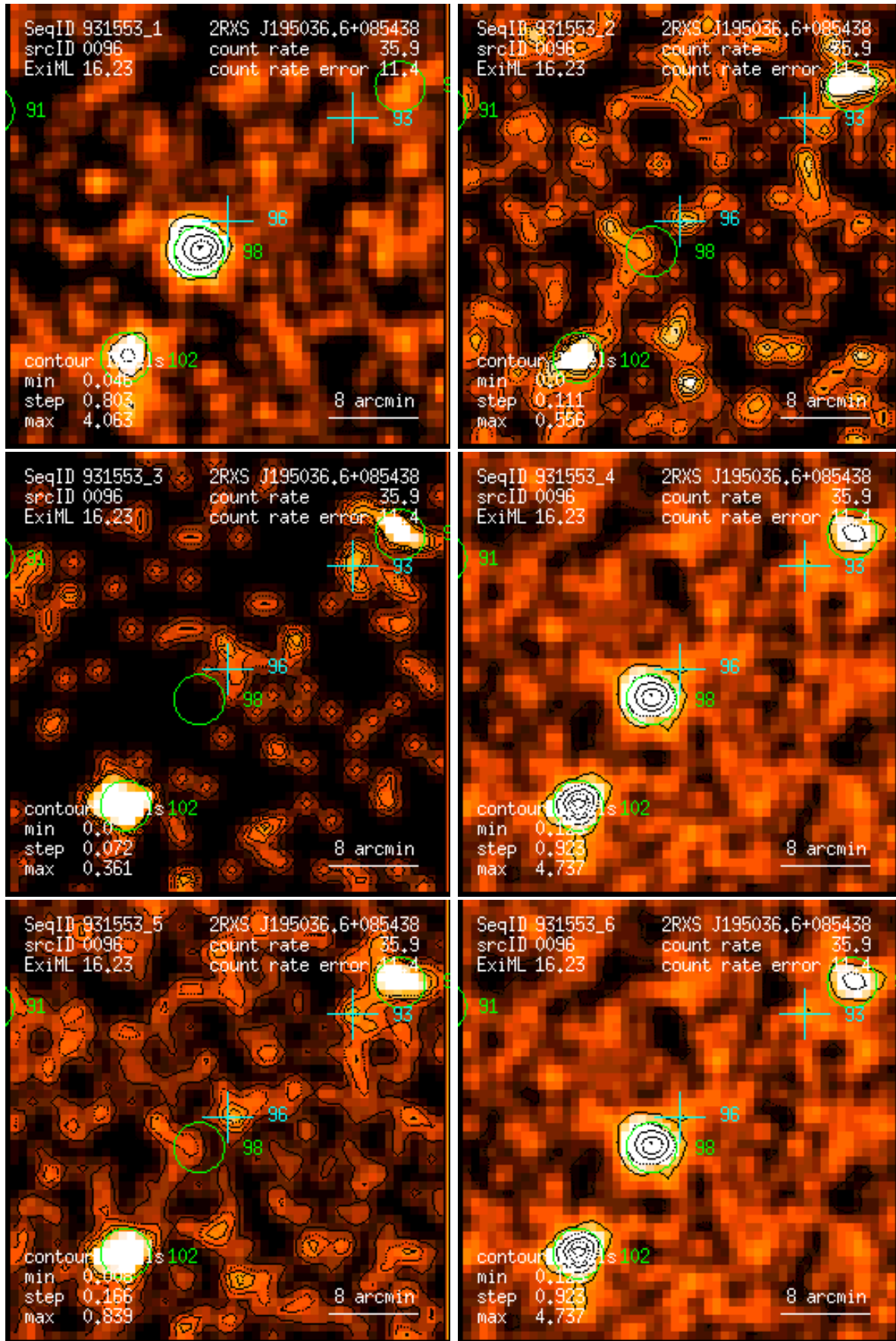
Figure 96: RASS 931553: detection 0096: band rate images, Gaussian filter: (1) PSPC channels 11 – 41, (2) 52 – 90, (3) 91 – 201, (4) 11 – 235, (5) 52 – 201, (6) 11 – 201. Broad band rates in counts/ks. Band rate contour levels in counts/ks/arcmin 2 .
