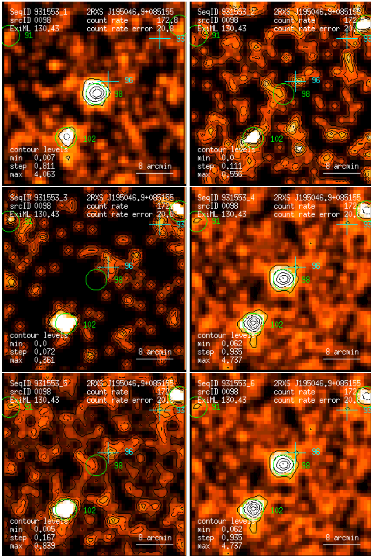
Figure 98: RASS 931553: detection 0098: band rate images, Gaussian filter: (1) PSPC channels 11 – 41, (2) 52 – 90, (3) 91 – 201, (4) 11 – 235, (5) 52 – 201, (6) 11 – 201. Broad band rates in counts/ks. Band rate contour levels in counts/ks/arcmin 2 .
