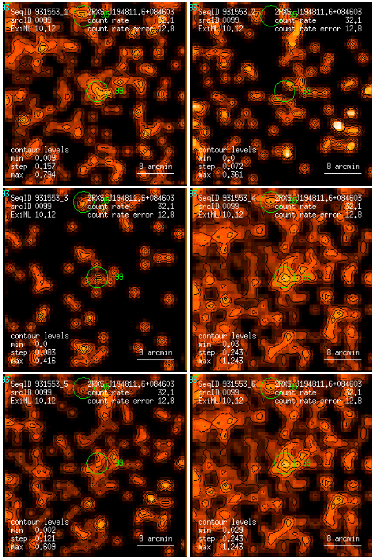
Figure 99: RASS 931553: detection 0099: band rate images, Gaussian filter: (1) PSPC channels 11 – 41, (2) 52 – 90, (3) 91 – 201, (4) 11 – 235, (5) 52 – 201, (6) 11 – 201. Broad band rates in counts/ks. Band rate contour levels in counts/ks/arcmin 2 .
