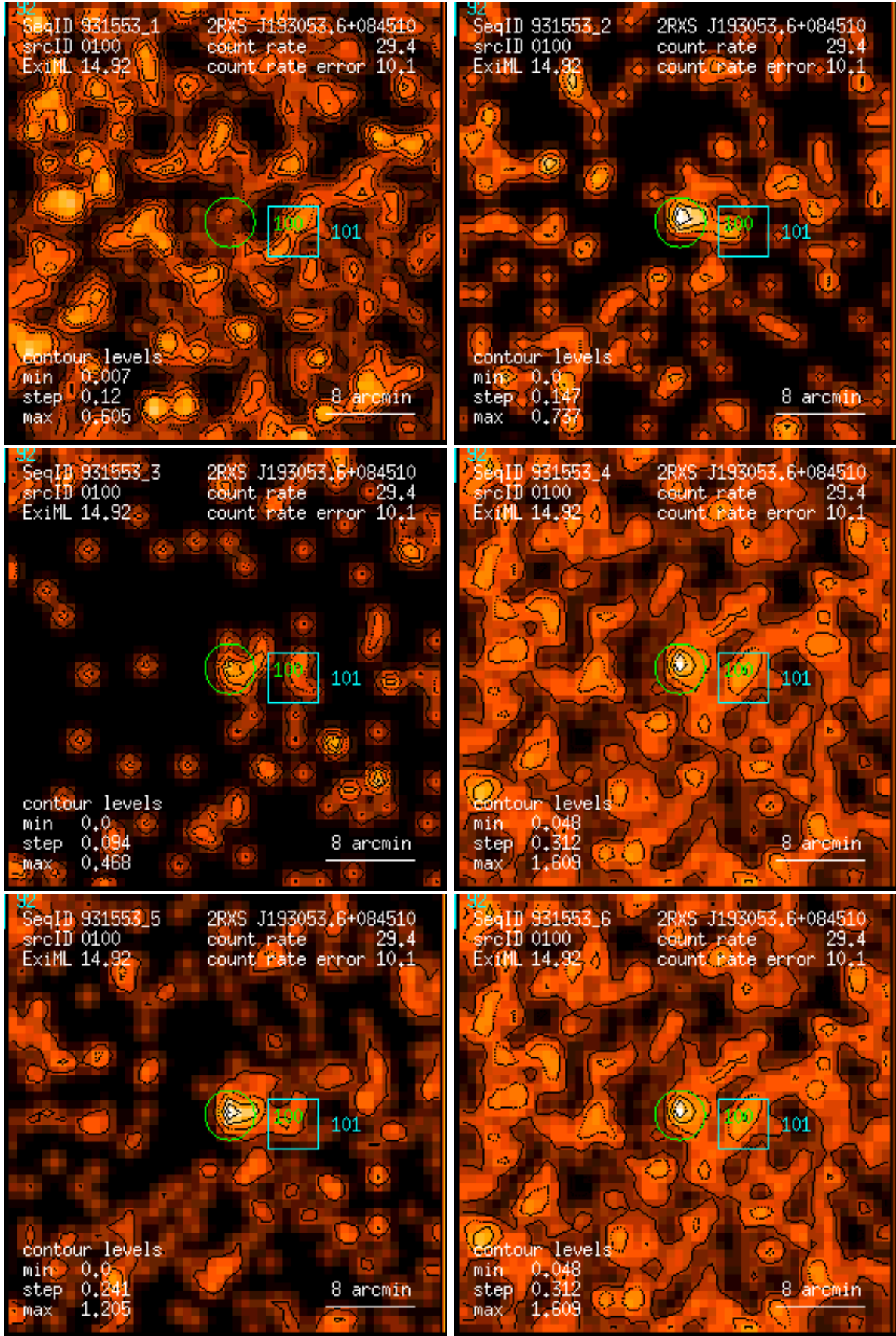
Figure 100: RASS 931553: detection 0100: band rate images, Gaussian filter: (1) PSPC channels 11 – 41, (2) 52 – 90, (3) 91 – 201, (4) 11 – 235, (5) 52 – 201, (6) 11 – 201. Broad band rates in counts/ks. Band rate contour levels in counts/ks/arcmin 2 .
