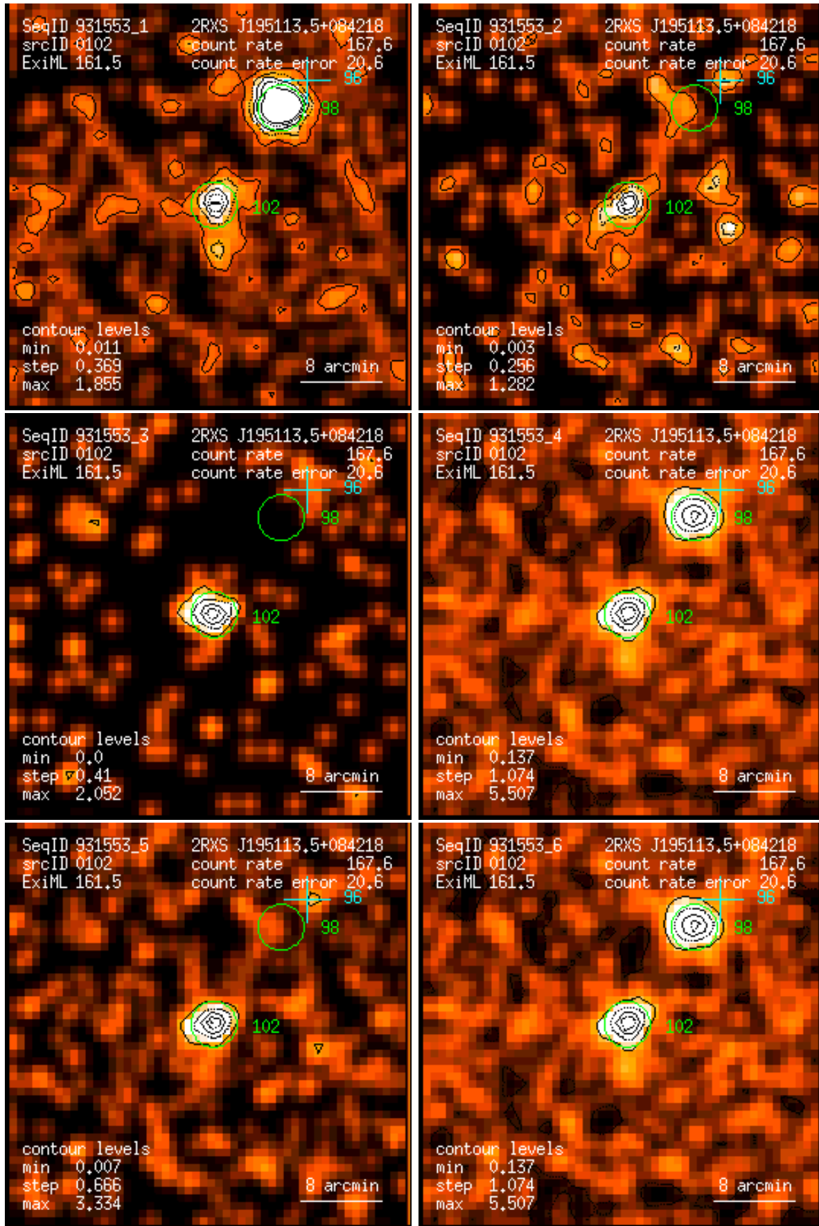
Figure 102: RASS 931553: detection 0102: band rate images, Gaussian filter: (1) PSPC channels 11 – 41, (2) 52 – 90, (3) 91 – 201, (4) 11 – 235, (5) 52 – 201, (6) 11 – 201. Broad band rates in counts/ks. Band rate contour levels in counts/ks/arcmin 2 .
