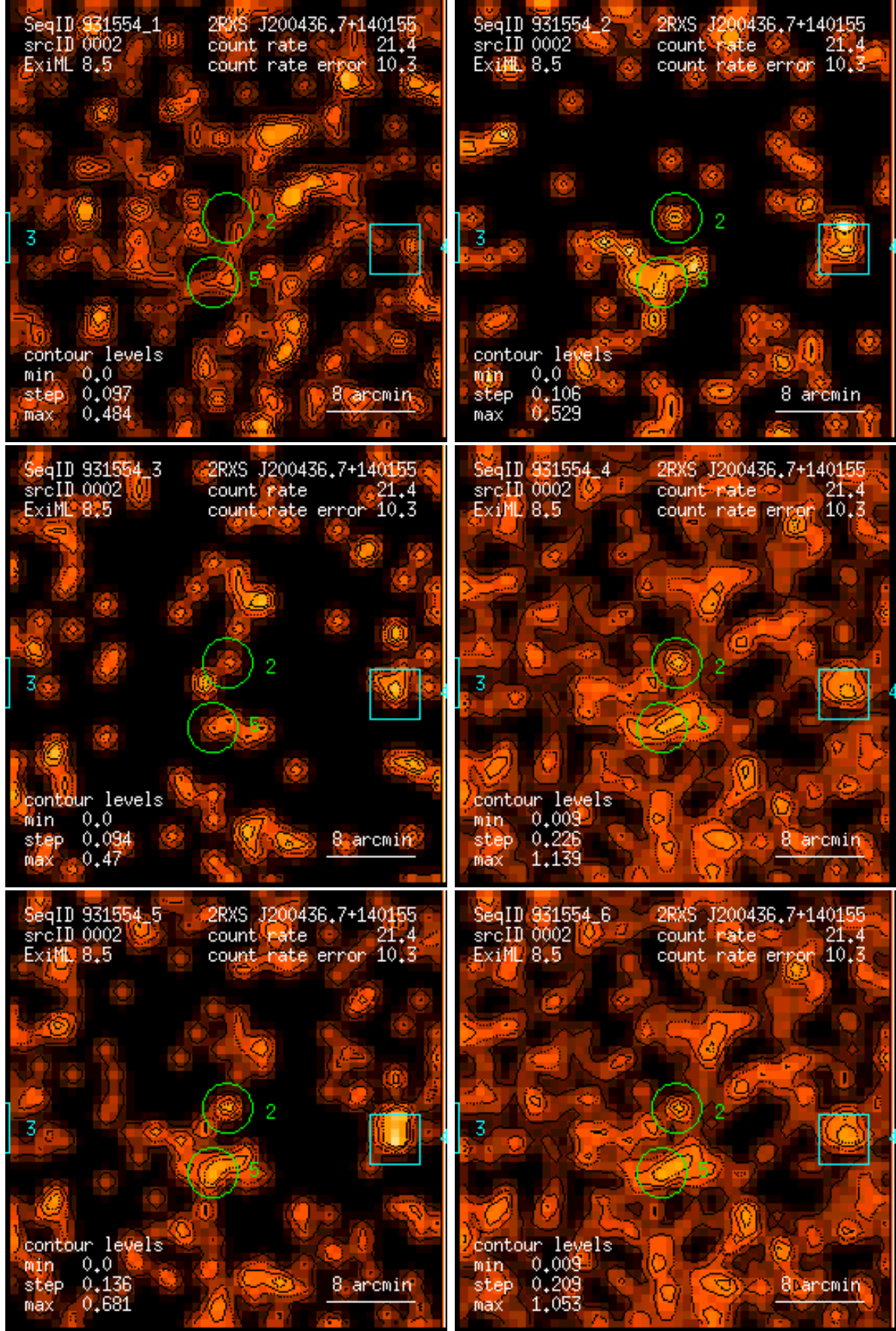
Figure 2: RASS 931554: detection 0002: band rate images, Gaussian filter: (1) PSPC channels 11 – 41, (2) 52 – 90, (3) 91 – 201, (4) 11 – 235, (5) 52 – 201, (6) 11 – 201. Broad band rates in counts/ks. Band rate contour levels in counts/ks/arcmin 2 .
