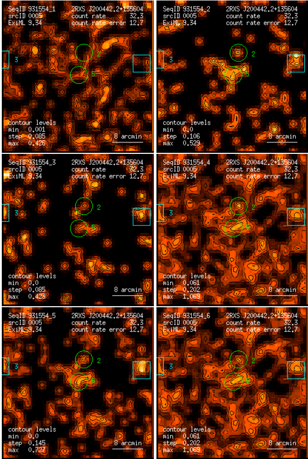
Figure 5: RASS 931554: detection 0005: band rate images, Gaussian filter: (1) PSPC channels 11 – 41, (2) 52 – 90, (3) 91 – 201, (4) 11 – 235, (5) 52 – 201, (6) 11 – 201. Broad band rates in counts/ks. Band rate contour levels in counts/ks/arcmin 2 .
