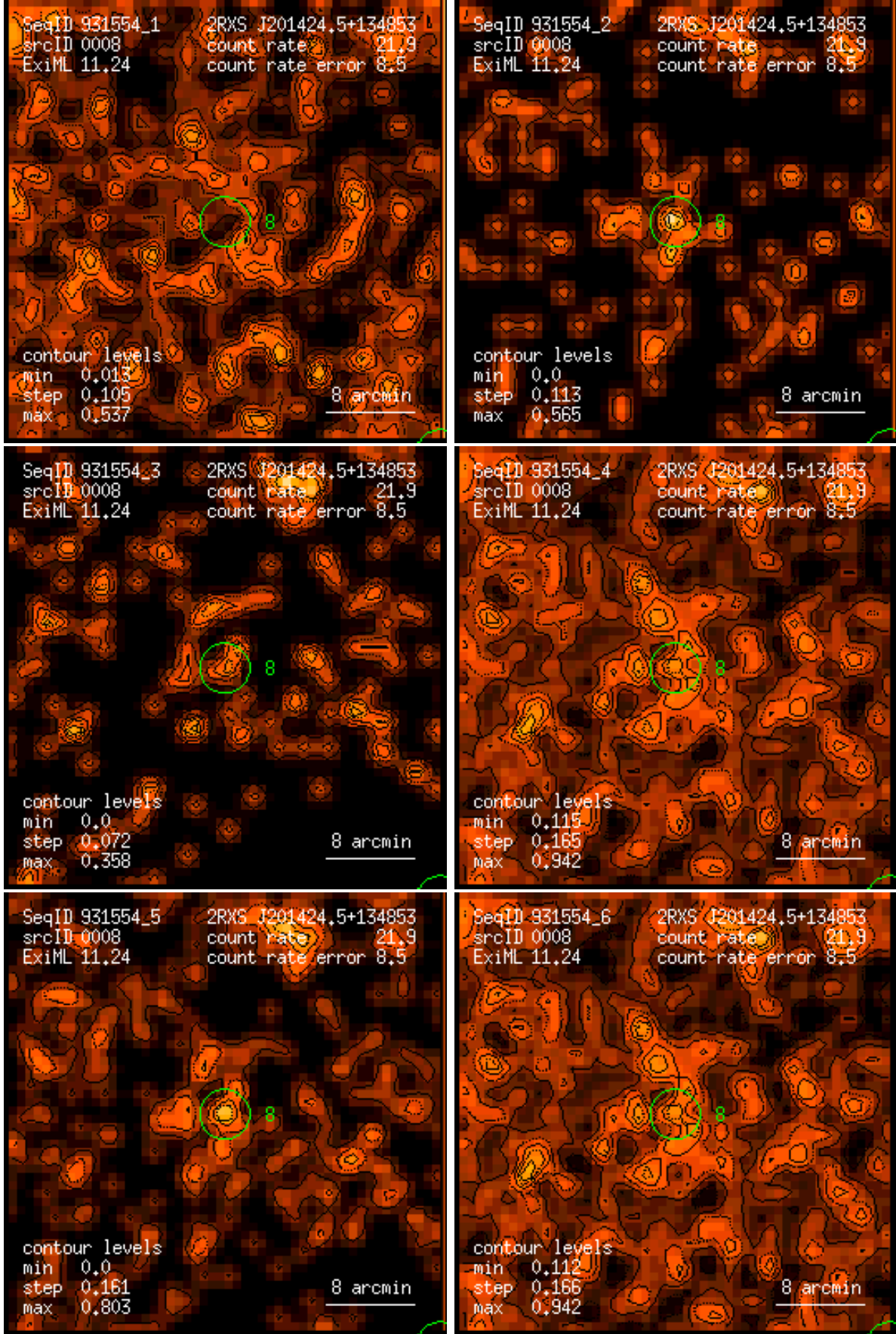
Figure 8: RASS 931554: detection 0008: band rate images, Gaussian filter: (1) PSPC channels 11 – 41, (2) 52 – 90, (3) 91 – 201, (4) 11 – 235, (5) 52 – 201, (6) 11 – 201. Broad band rates in counts/ks. Band rate contour levels in counts/ks/arcmin 2 .
