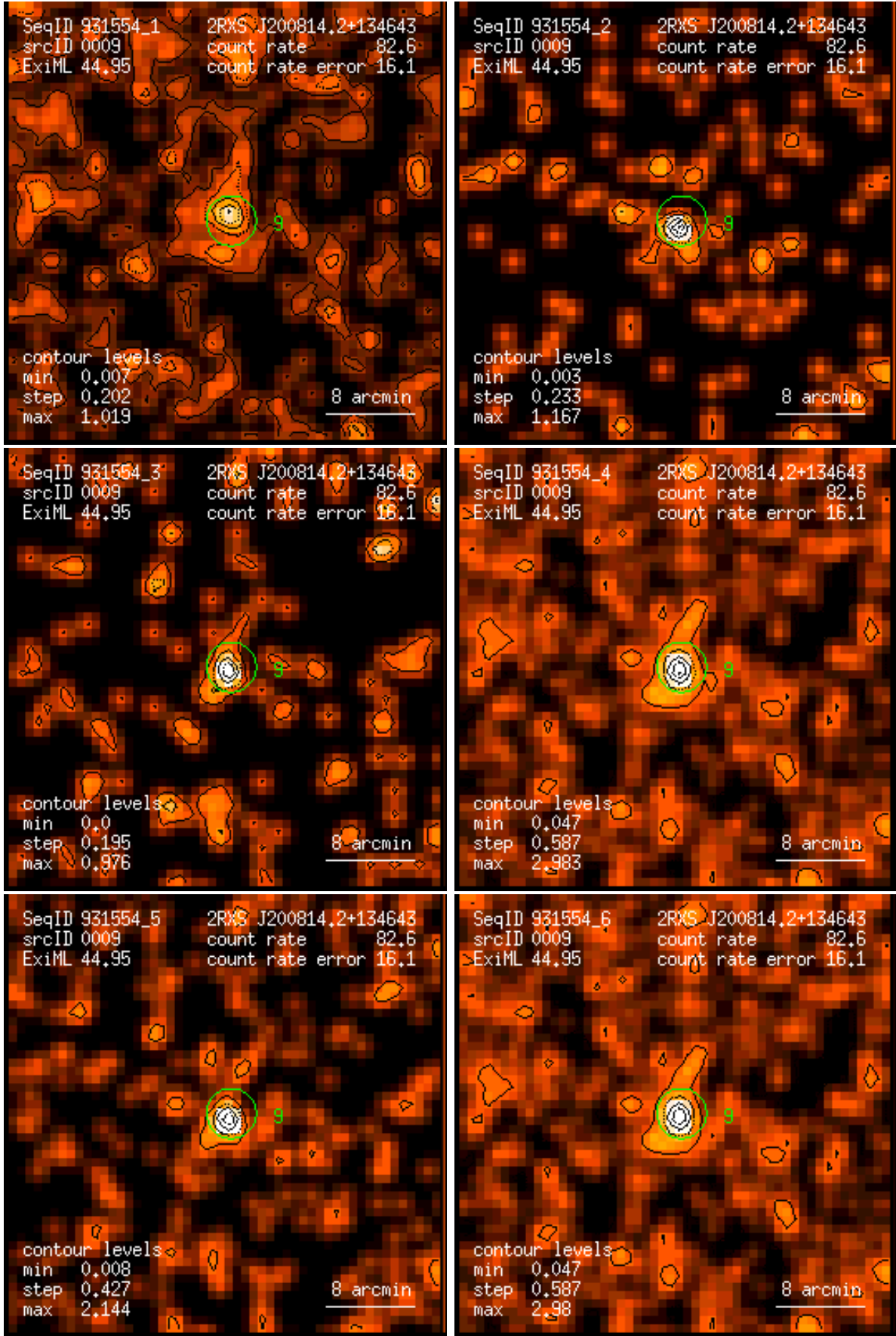
Figure 9: RASS 931554: detection 0009: band rate images, Gaussian filter: (1) PSPC channels 11 – 41, (2) 52 – 90, (3) 91 – 201, (4) 11 – 235, (5) 52 – 201, (6) 11 – 201. Broad band rates in counts/ks. Band rate contour levels in counts/ks/arcmin 2 .
