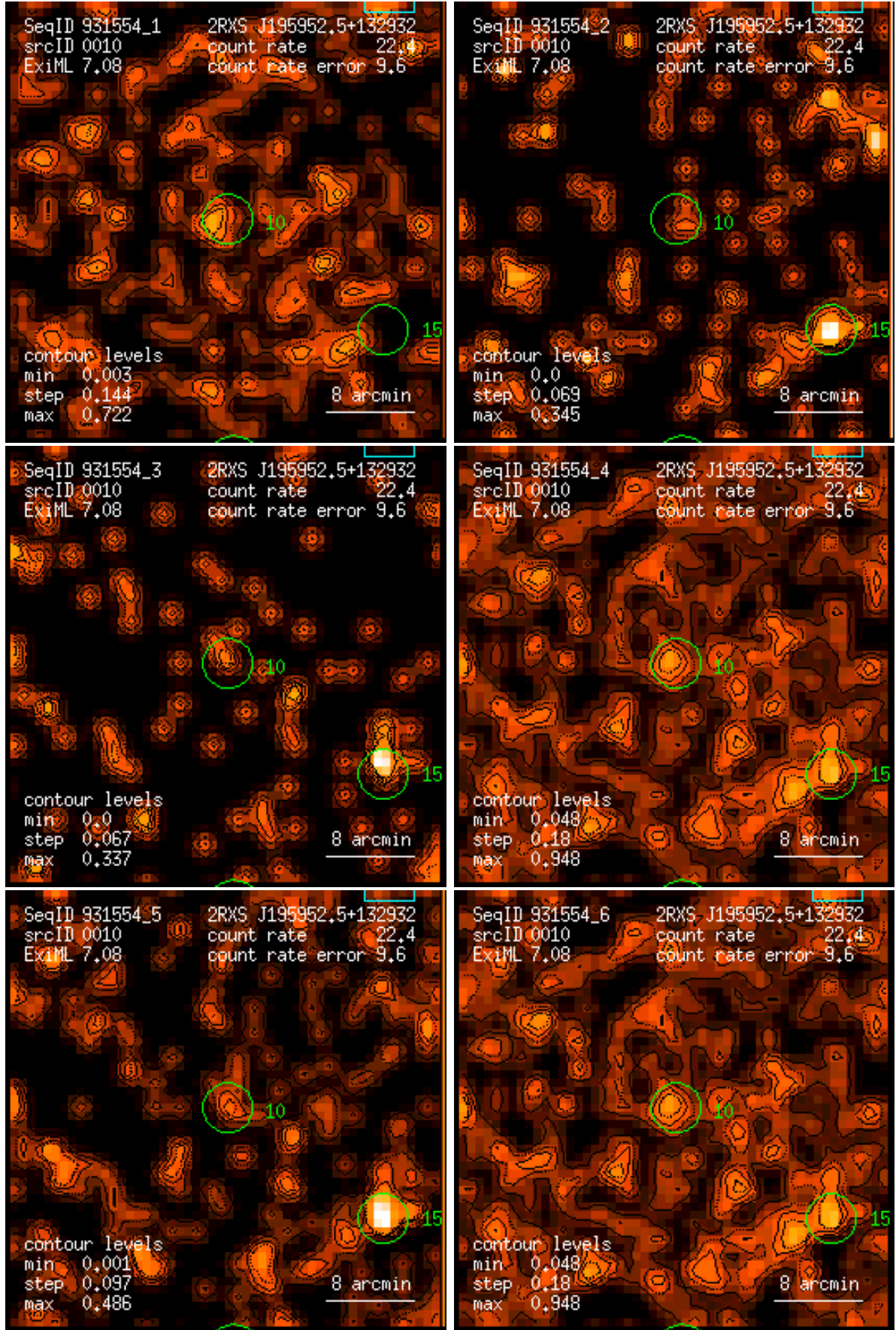
Figure 10: RASS 931554: detection 0010: band rate images, Gaussian filter: (1) PSPC channels 11 – 41, (2) 52 – 90, (3) 91 – 201, (4) 11 – 235, (5) 52 – 201, (6) 11 – 201. Broad band rates in counts/ks. Band rate contour levels in counts/ks/arcmin 2 .
