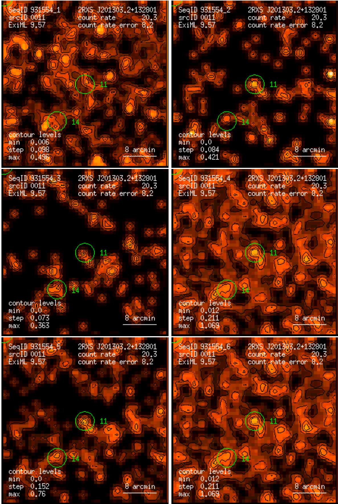
Figure 11: RASS 931554: detection 0011: band rate images, Gaussian filter: (1) PSPC channels 11 – 41, (2) 52 – 90, (3) 91 – 201, (4) 11 – 235, (5) 52 – 201, (6) 11 – 201. Broad band rates in counts/ks. Band rate contour levels in counts/ks/arcmin 2 .
