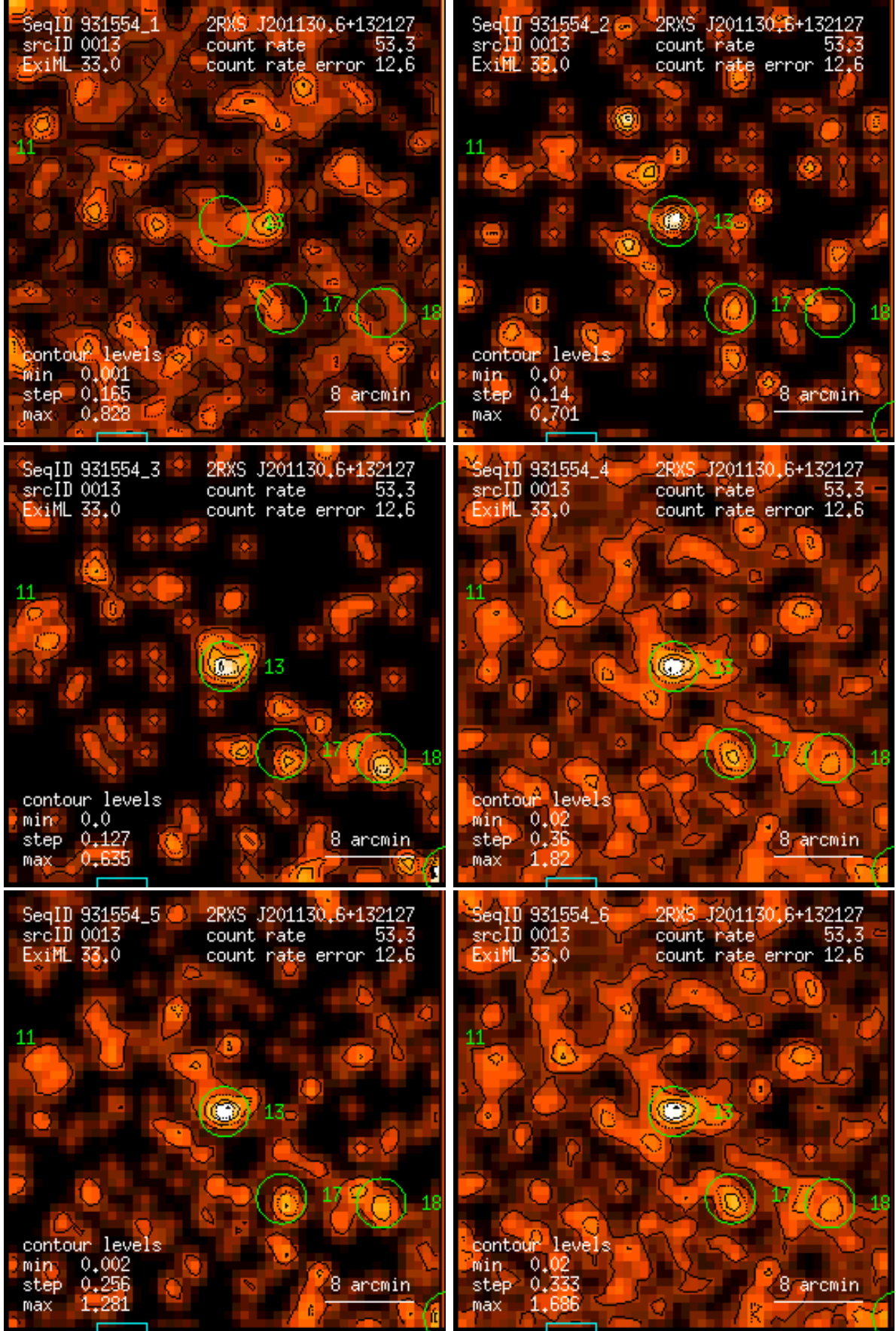
Figure 13: RASS 931554: detection 0013: band rate images, Gaussian filter: (1) PSPC channels 11 – 41, (2) 52 – 90, (3) 91 – 201, (4) 11 – 235, (5) 52 – 201, (6) 11 – 201. Broad band rates in counts/ks. Band rate contour levels in counts/ks/arcmin 2 .
