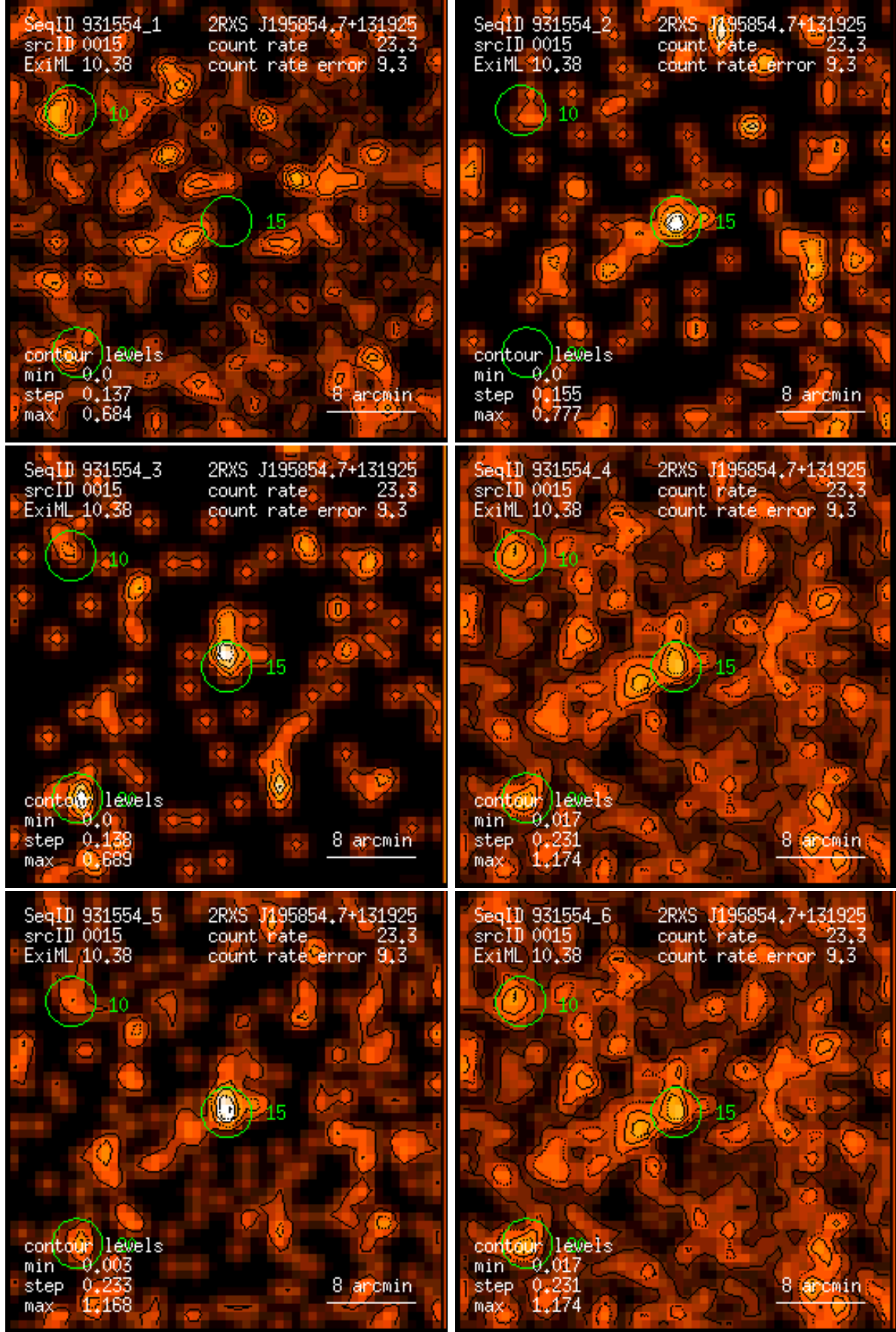
Figure 15: RASS 931554: detection 0015: band rate images, Gaussian filter: (1) PSPC channels 11 – 41, (2) 52 – 90, (3) 91 – 201, (4) 11 – 235, (5) 52 – 201, (6) 11 – 201. Broad band rates in counts/ks. Band rate contour levels in counts/ks/arcmin 2 .
