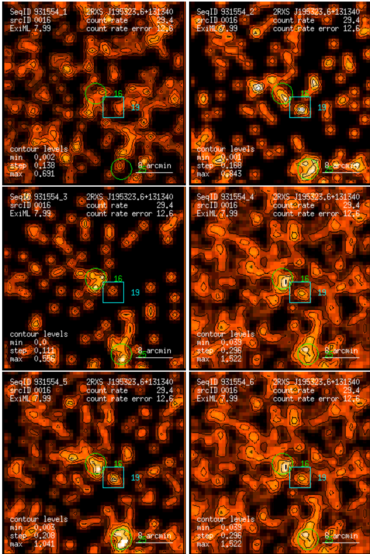
Figure 16: RASS 931554: detection 0016: band rate images, Gaussian filter: (1) PSPC channels 11 – 41, (2) 52 – 90, (3) 91 – 201, (4) 11 – 235, (5) 52 – 201, (6) 11 – 201. Broad band rates in counts/ks. Band rate contour levels in counts/ks/arcmin 2 .
