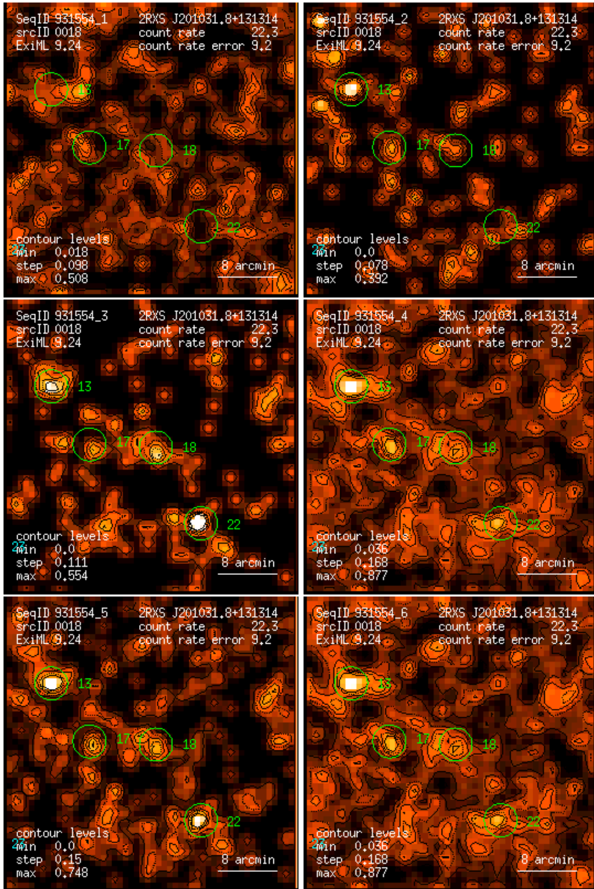
Figure 18: RASS 931554: detection 0018: band rate images, Gaussian filter: (1) PSPC channels 11 – 41, (2) 52 – 90, (3) 91 – 201, (4) 11 – 235, (5) 52 – 201, (6) 11 – 201. Broad band rates in counts/ks. Band rate contour levels in counts/ks/arcmin 2 .
