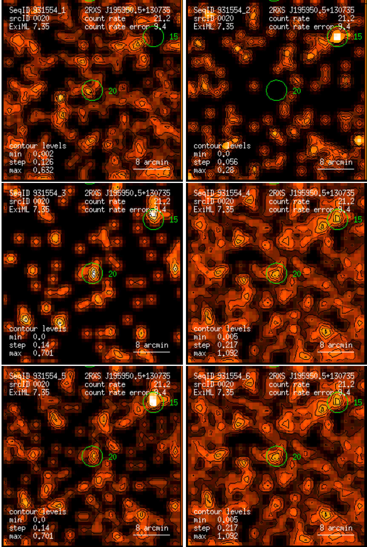
Figure 20: RASS 931554: detection 0020: band rate images, Gaussian filter: (1) PSPC channels 11 – 41, (2) 52 – 90, (3) 91 – 201, (4) 11 – 235, (5) 52 – 201, (6) 11 – 201. Broad band rates in counts/ks. Band rate contour levels in counts/ks/arcmin 2 .
