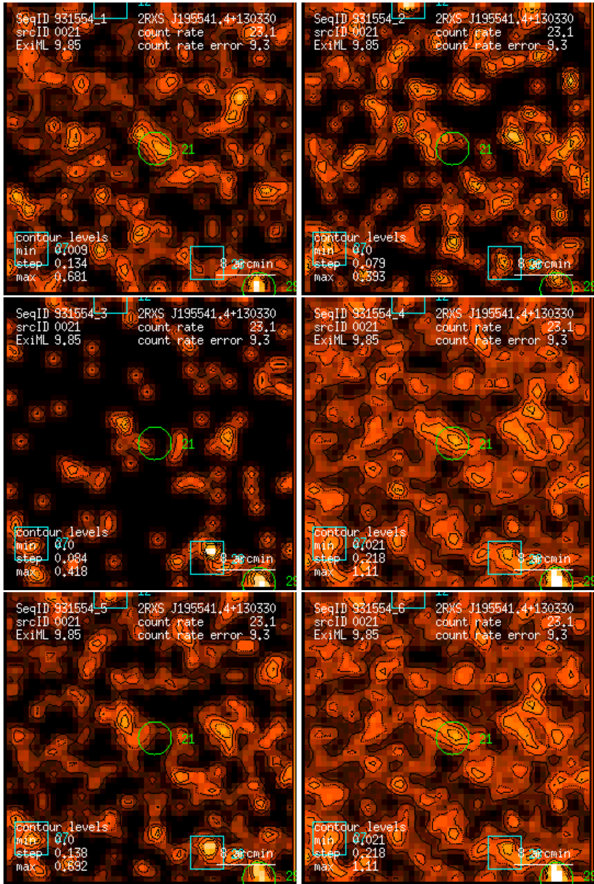
Figure 21: RASS 931554: detection 0021: band rate images, Gaussian filter: (1) PSPC channels 11 – 41, (2) 52 – 90, (3) 91 – 201, (4) 11 – 235, (5) 52 – 201, (6) 11 – 201. Broad band rates in counts/ks. Band rate contour levels in counts/ks/arcmin 2 .
