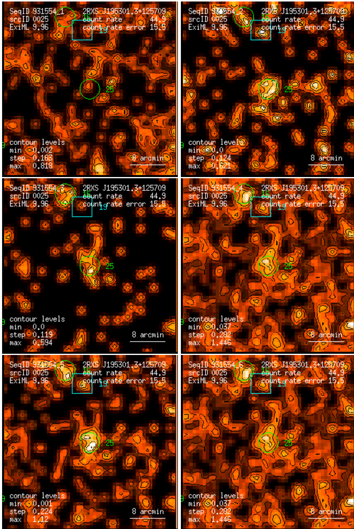
Figure 25: RASS 931554: detection 0025: band rate images, Gaussian filter: (1) PSPC channels 11 – 41, (2) 52 – 90, (3) 91 – 201, (4) 11 – 235, (5) 52 – 201, (6) 11 – 201. Broad band rates in counts/ks. Band rate contour levels in counts/ks/arcmin 2 .
