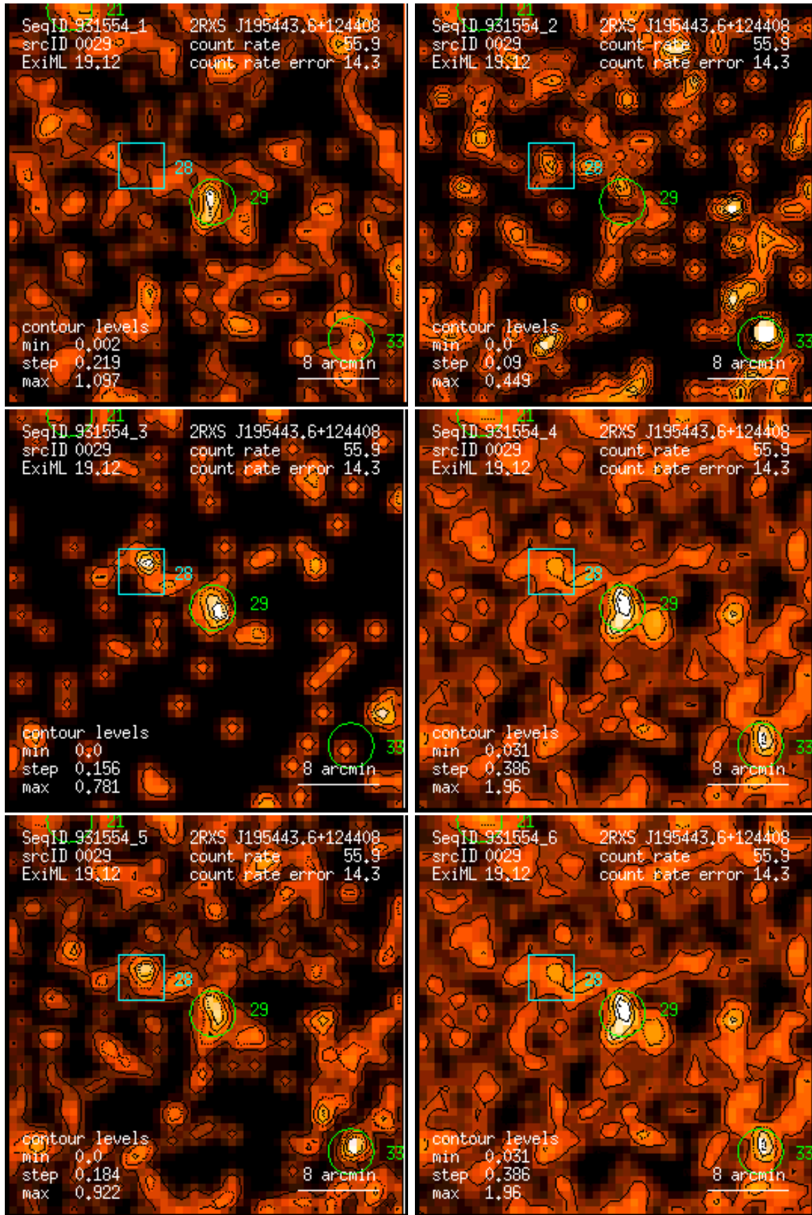
Figure 29: RASS 931554: detection 0029: band rate images, Gaussian filter: (1) PSPC channels 11 – 41, (2) 52 – 90, (3) 91 – 201, (4) 11 – 235, (5) 52 – 201, (6) 11 – 201. Broad band rates in counts/ks. Band rate contour levels in counts/ks/arcmin 2 .
