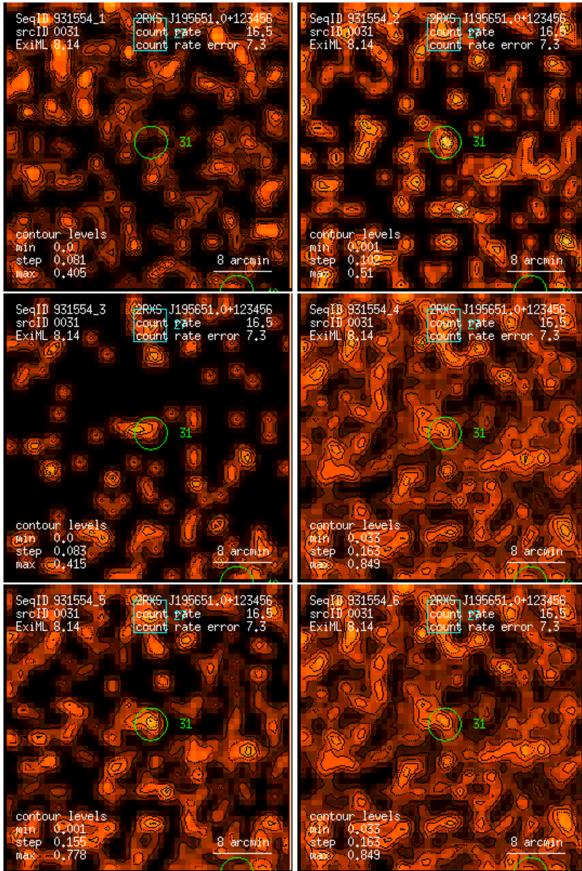
Figure 31: RASS 931554: detection 0031: band rate images, Gaussian filter: (1) PSPC channels 11 – 41, (2) 52 – 90, (3) 91 – 201, (4) 11 – 235, (5) 52 – 201, (6) 11 – 201. Broad band rates in counts/ks. Band rate contour levels in counts/ks/arcmin 2 .
