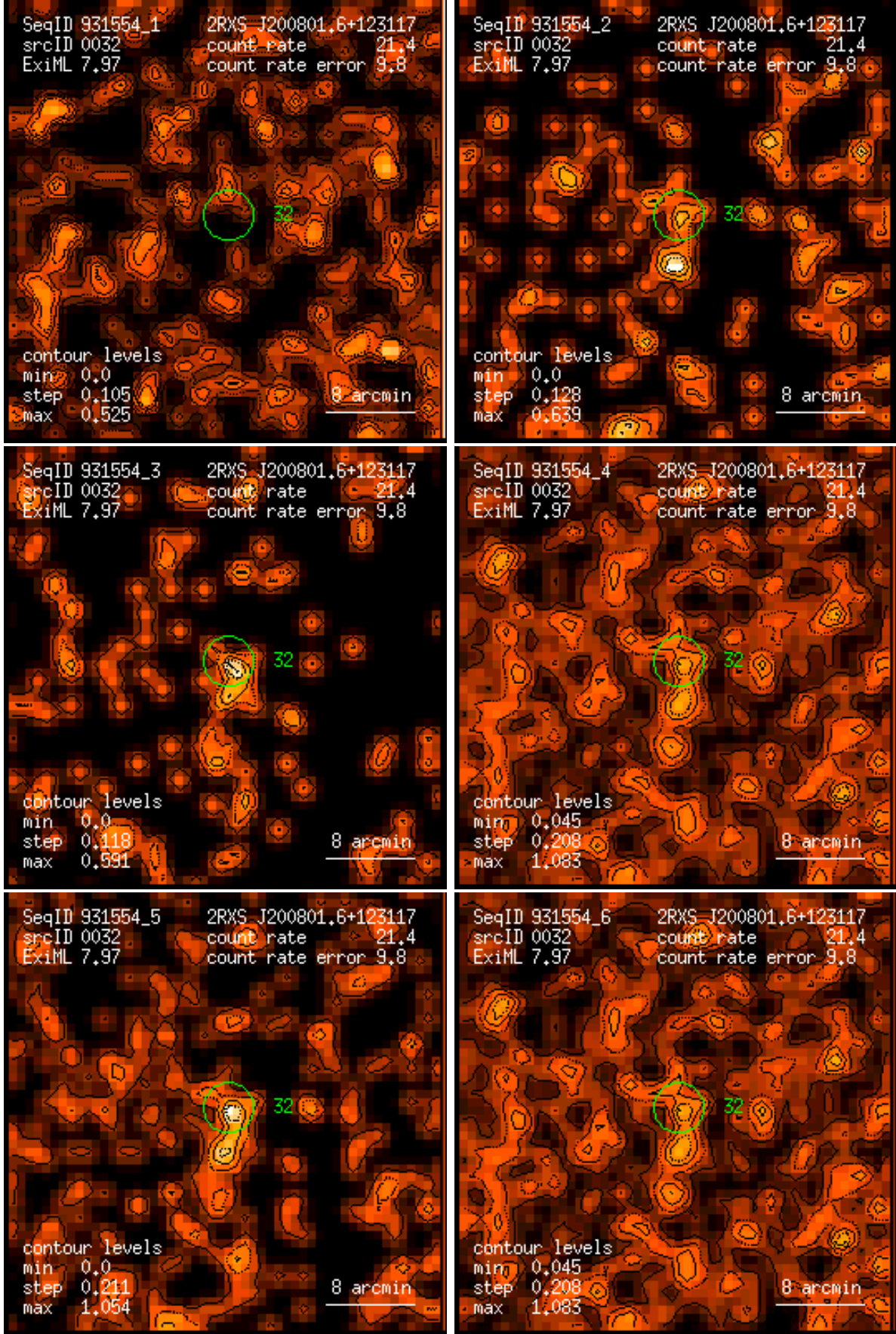
Figure 32: RASS 931554: detection 0032: band rate images, Gaussian filter: (1) PSPC channels 11 – 41, (2) 52 – 90, (3) 91 – 201, (4) 11 – 235, (5) 52 – 201, (6) 11 – 201. Broad band rates in counts/ks. Band rate contour levels in counts/ks/arcmin 2 .
