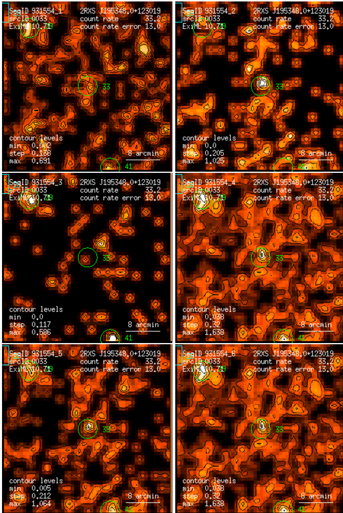
Figure 33: RASS 931554: detection 0033: band rate images, Gaussian filter: (1) PSPC channels 11 – 41, (2) 52 – 90, (3) 91 – 201, (4) 11 – 235, (5) 52 – 201, (6) 11 – 201. Broad band rates in counts/ks. Band rate contour levels in counts/ks/arcmin 2 .
