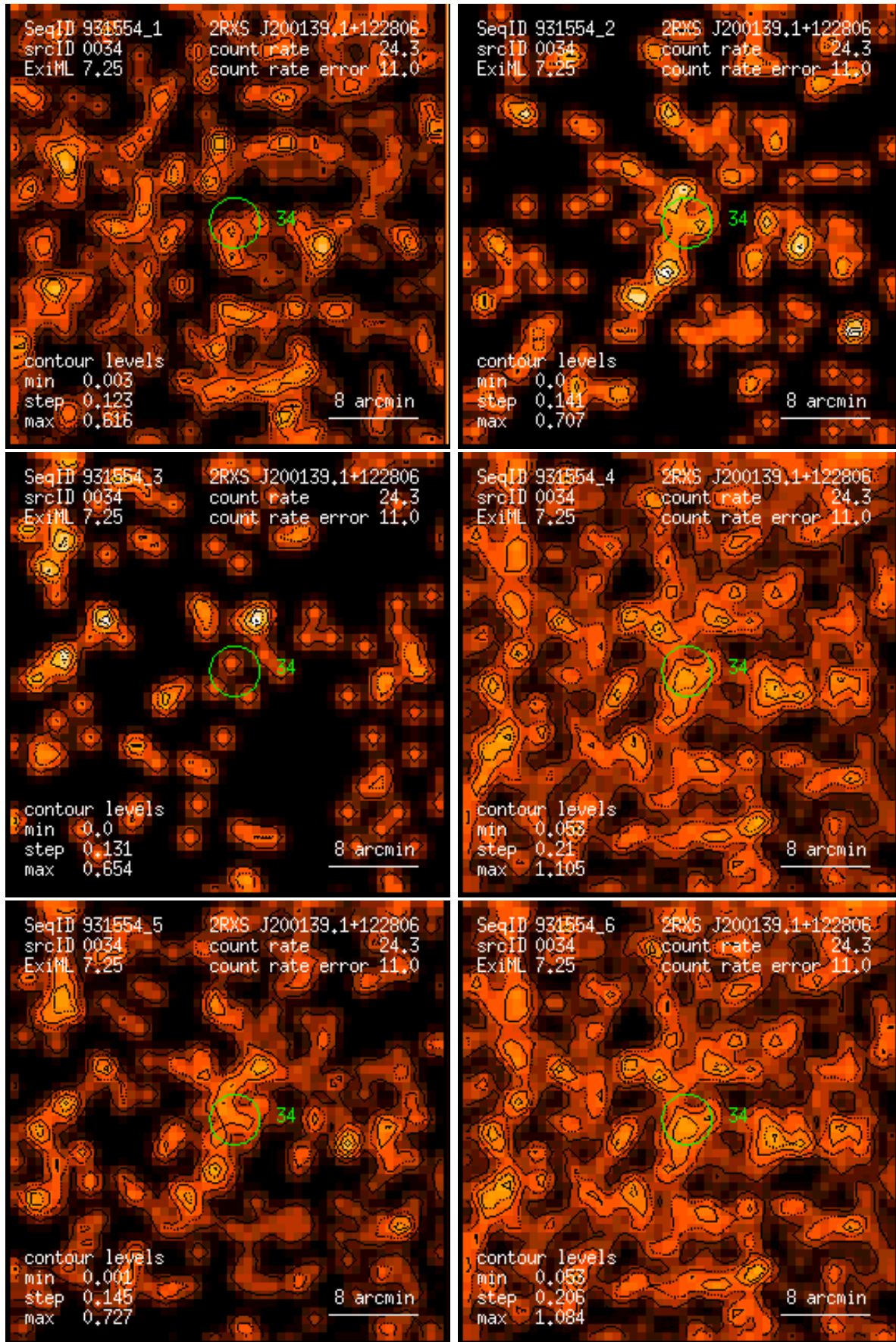
Figure 34: RASS 931554: detection 0034: band rate images, Gaussian filter: (1) PSPC channels 11 – 41, (2) 52 – 90, (3) 91 – 201, (4) 11 – 235, (5) 52 – 201, (6) 11 – 201. Broad band rates in counts/ks. Band rate contour levels in counts/ks/arcmin 2 .
