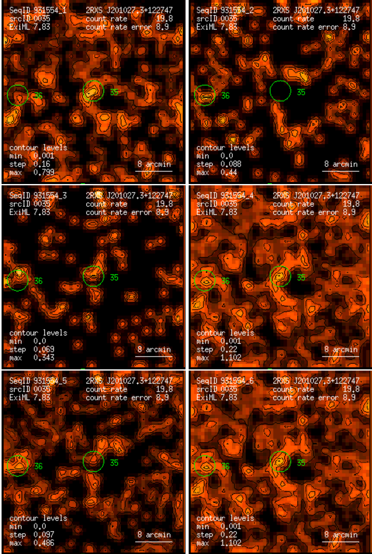
Figure 35: RASS 931554: detection 0035: band rate images, Gaussian filter: (1) PSPC channels 11 – 41, (2) 52 – 90, (3) 91 – 201, (4) 11 – 235, (5) 52 – 201, (6) 11 – 201. Broad band rates in counts/ks. Band rate contour levels in counts/ks/arcmin 2 .
