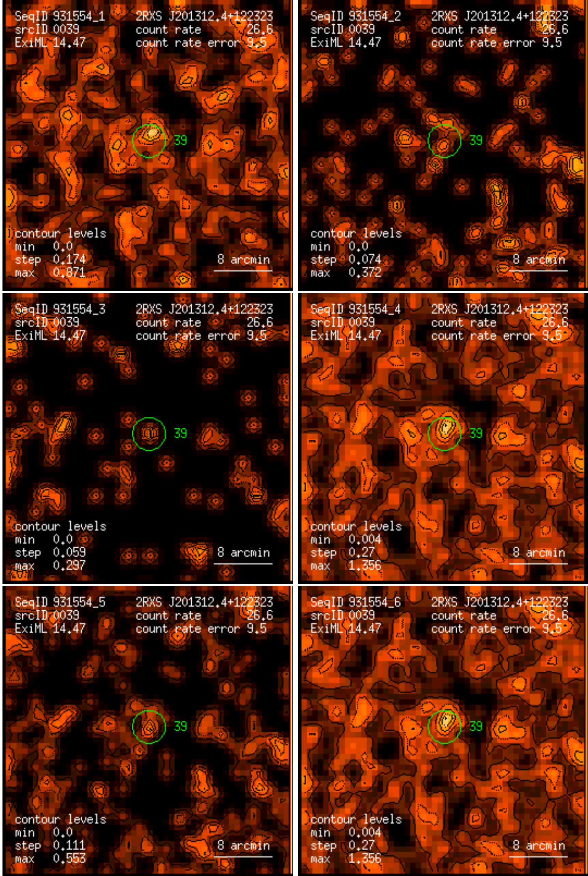
Figure 39: RASS 931554: detection 0039: band rate images, Gaussian filter: (1) PSPC channels 11 – 41, (2) 52 – 90, (3) 91 – 201, (4) 11 – 235, (5) 52 – 201, (6) 11 – 201. Broad band rates in counts/ks. Band rate contour levels in counts/ks/arcmin 2 .
