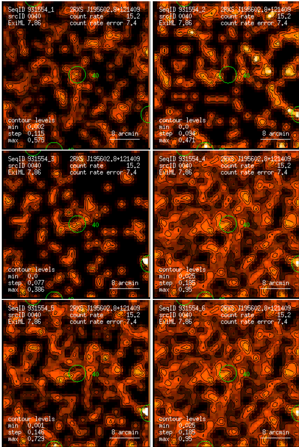
Figure 40: RASS 931554: detection 0040: band rate images, Gaussian filter: (1) PSPC channels 11 – 41, (2) 52 – 90, (3) 91 – 201, (4) 11 – 235, (5) 52 – 201, (6) 11 – 201. Broad band rates in counts/ks. Band rate contour levels in counts/ks/arcmin 2 .
