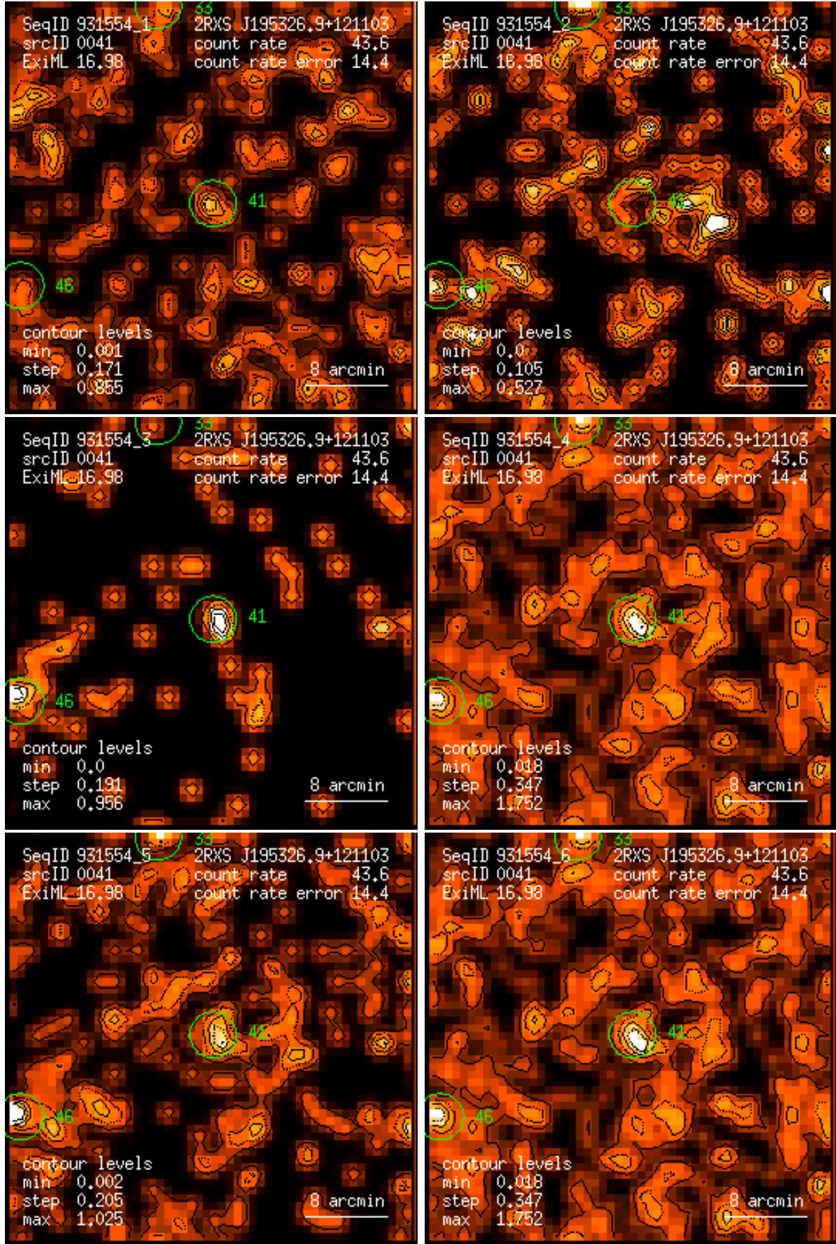
Figure 41: RASS 931554: detection 0041: band rate images, Gaussian filter: (1) PSPC channels 11 – 41, (2) 52 – 90, (3) 91 – 201, (4) 11 – 235, (5) 52 – 201, (6) 11 – 201. Broad band rates in counts/ks. Band rate contour levels in counts/ks/arcmin 2 .
