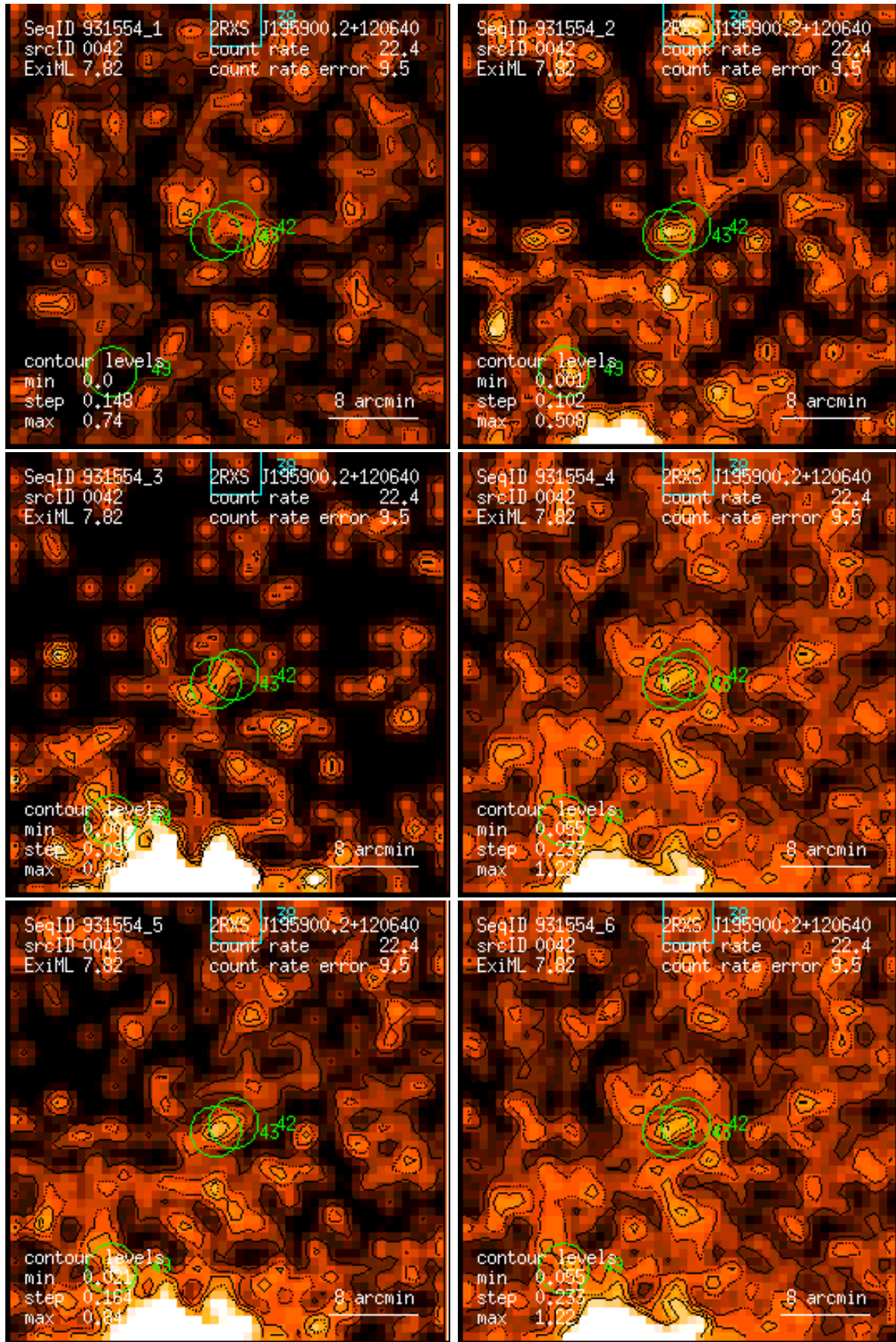
Figure 42: RASS 931554: detection 0042: band rate images, Gaussian filter: (1) PSPC channels 11 – 41, (2) 52 – 90, (3) 91 – 201, (4) 11 – 235, (5) 52 – 201, (6) 11 – 201. Broad band rates in counts/ks. Band rate contour levels in counts/ks/arcmin 2 .
