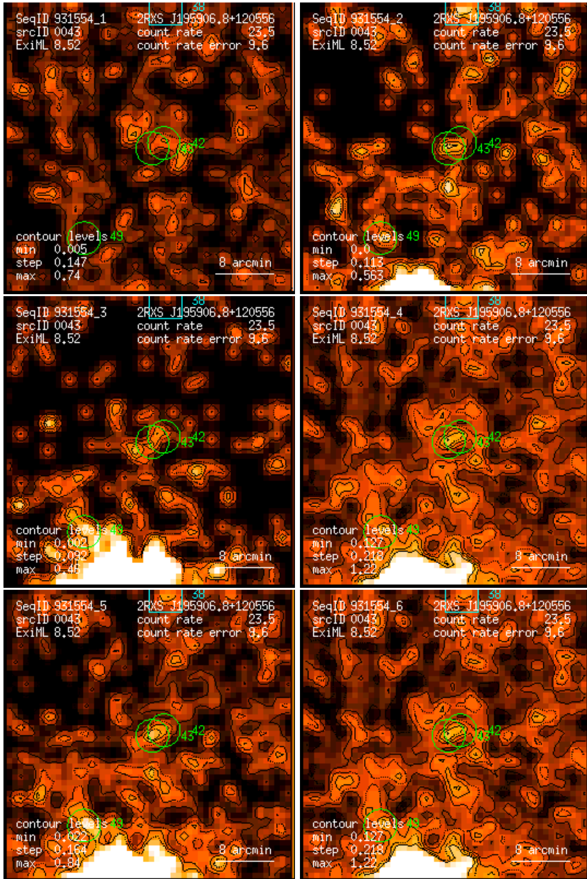
Figure 43: RASS 931554: detection 0043: band rate images, Gaussian filter: (1) PSPC channels 11 – 41, (2) 52 – 90, (3) 91 – 201, (4) 11 – 235, (5) 52 – 201, (6) 11 – 201. Broad band rates in counts/ks. Band rate contour levels in counts/ks/arcmin 2 .
