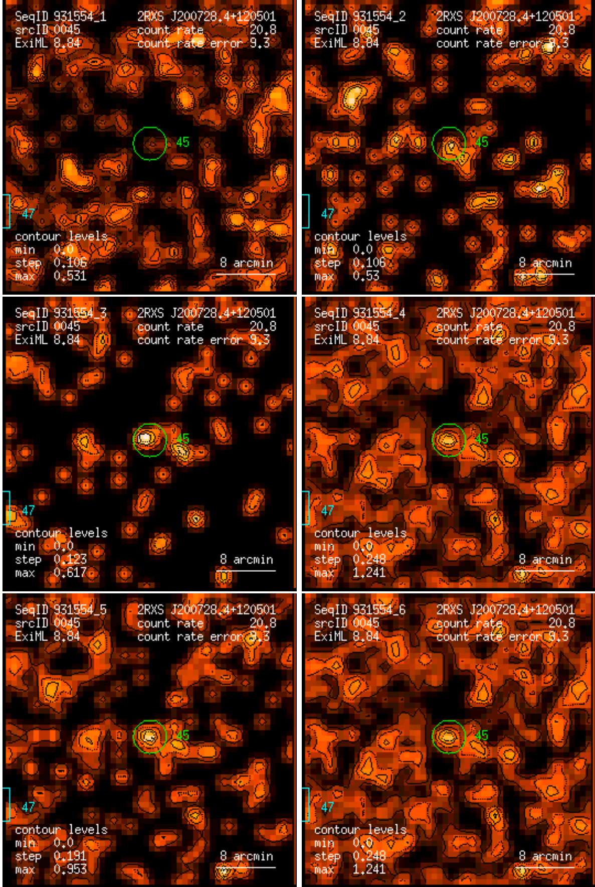
Figure 45: RASS 931554: detection 0045: band rate images, Gaussian filter: (1) PSPC channels 11 – 41, (2) 52 – 90, (3) 91 – 201, (4) 11 – 235, (5) 52 – 201, (6) 11 – 201. Broad band rates in counts/ks. Band rate contour levels in counts/ks/arcmin 2 .
