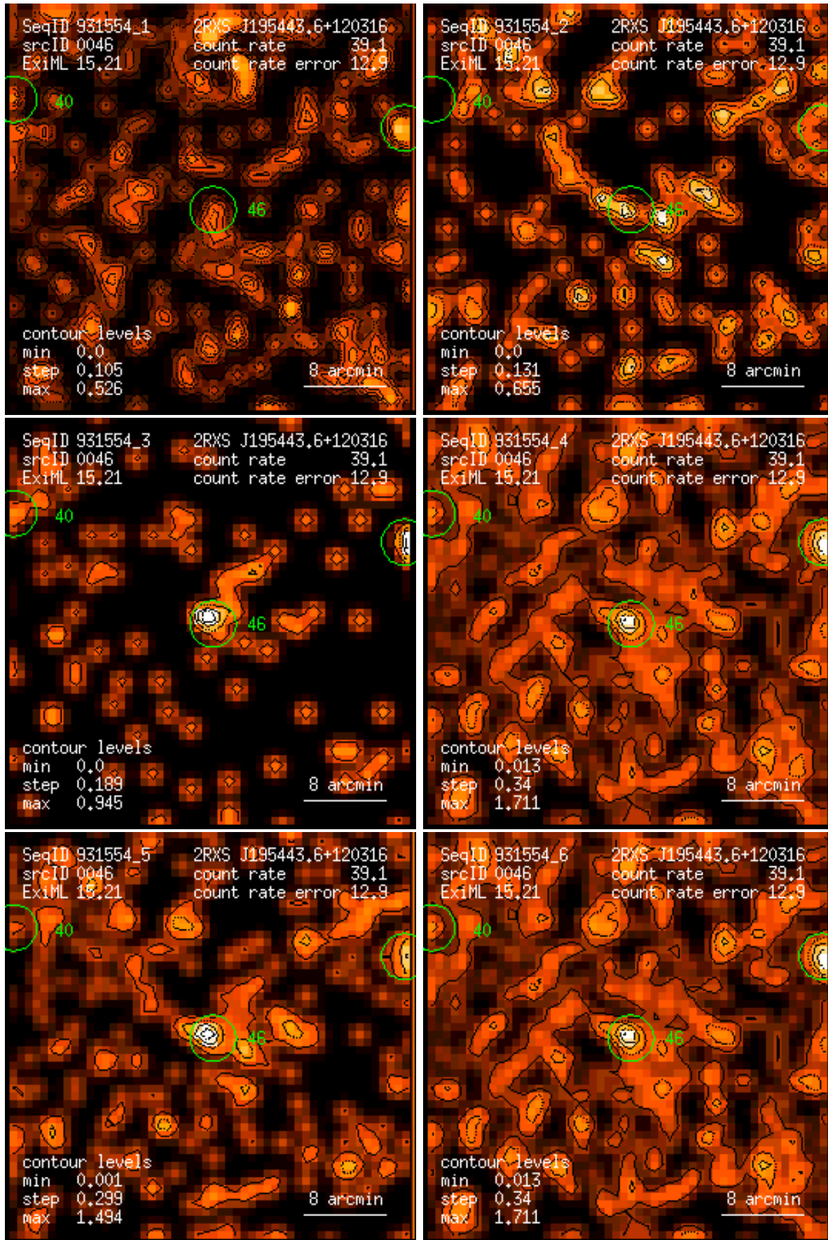
Figure 46: RASS 931554: detection 0046: band rate images, Gaussian filter: (1) PSPC channels 11 – 41, (2) 52 – 90, (3) 91 – 201, (4) 11 – 235, (5) 52 – 201, (6) 11 – 201. Broad band rates in counts/ks. Band rate contour levels in counts/ks/arcmin 2 .
