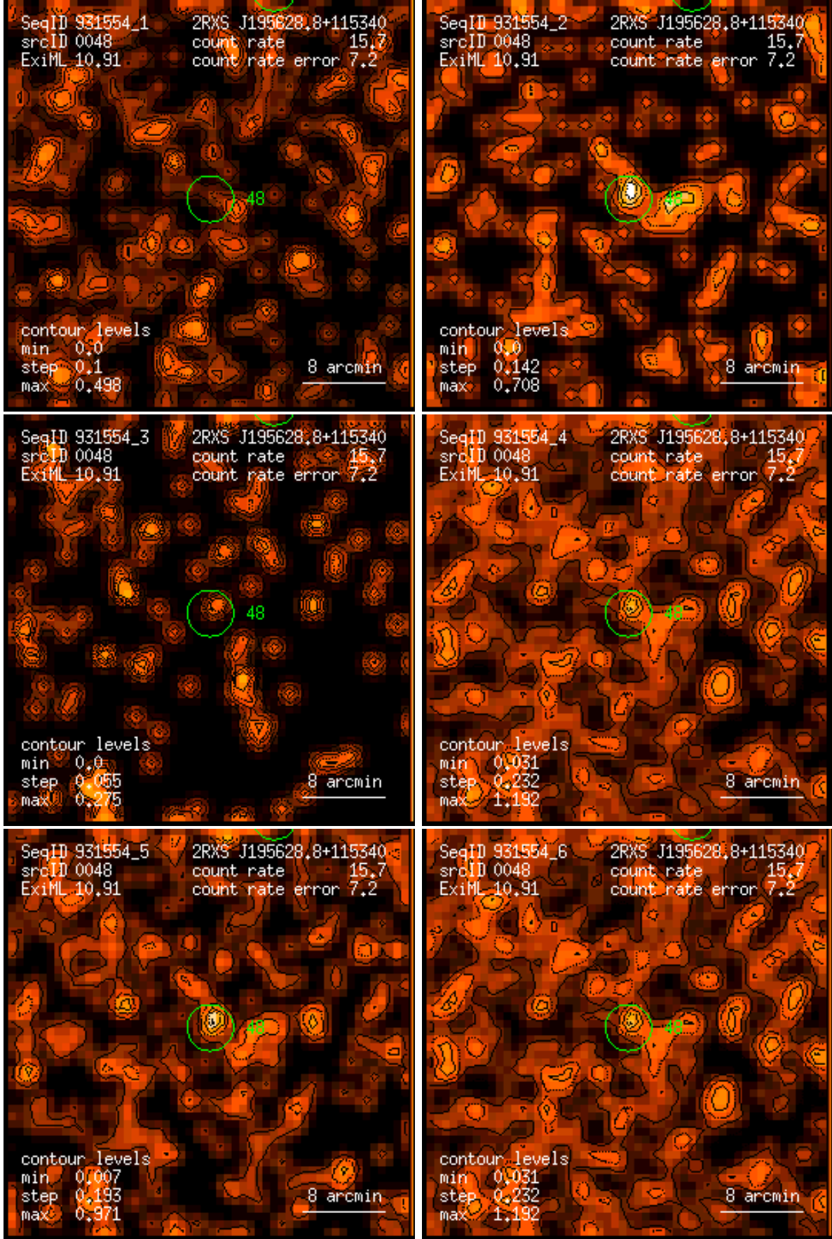
Figure 48: RASS 931554: detection 0048: band rate images, Gaussian filter: (1) PSPC channels 11 – 41, (2) 52 – 90, (3) 91 – 201, (4) 11 – 235, (5) 52 – 201, (6) 11 – 201. Broad band rates in counts/ks. Band rate contour levels in counts/ks/arcmin 2 .
