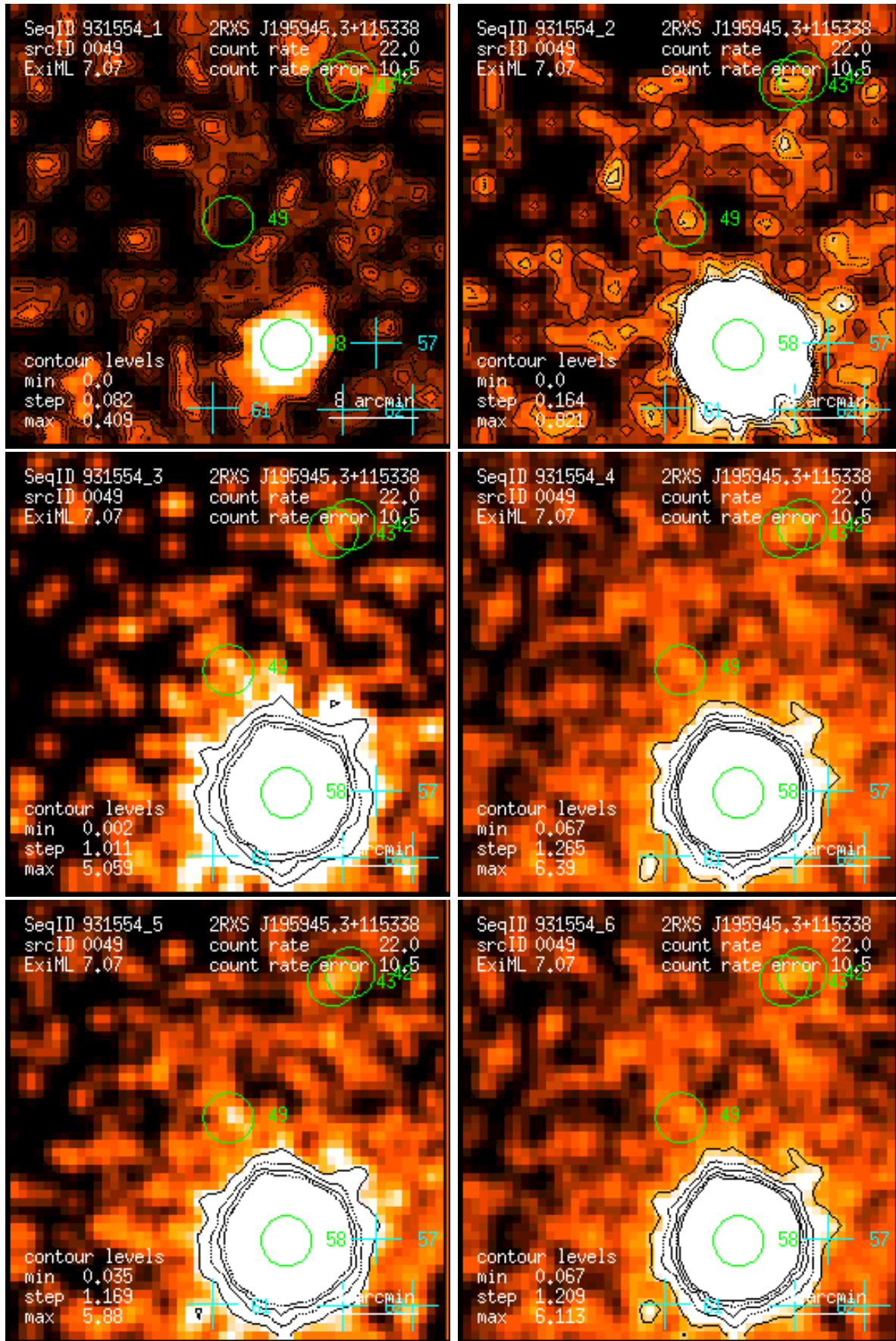
Figure 49: RASS 931554: detection 0049: band rate images, Gaussian filter: (1) PSPC channels 11 – 41, (2) 52 – 90, (3) 91 – 201, (4) 11 – 235, (5) 52 – 201, (6) 11 – 201. Broad band rates in counts/ks. Band rate contour levels in counts/ks/arcmin 2 .
