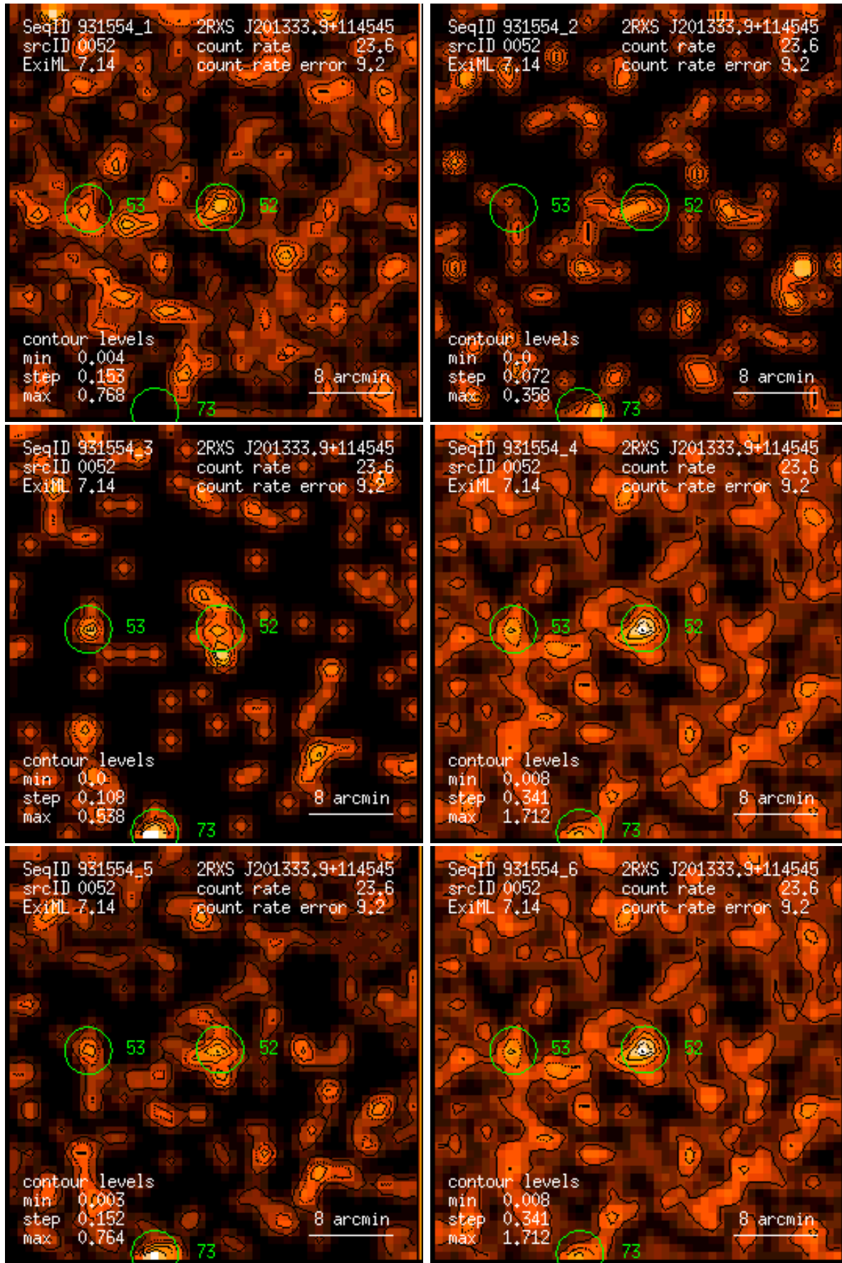
Figure 52: RASS 931554: detection 0052: band rate images, Gaussian filter: (1) PSPC channels 11 – 41, (2) 52 – 90, (3) 91 – 201, (4) 11 – 235, (5) 52 – 201, (6) 11 – 201. Broad band rates in counts/ks. Band rate contour levels in counts/ks/arcmin 2 .
