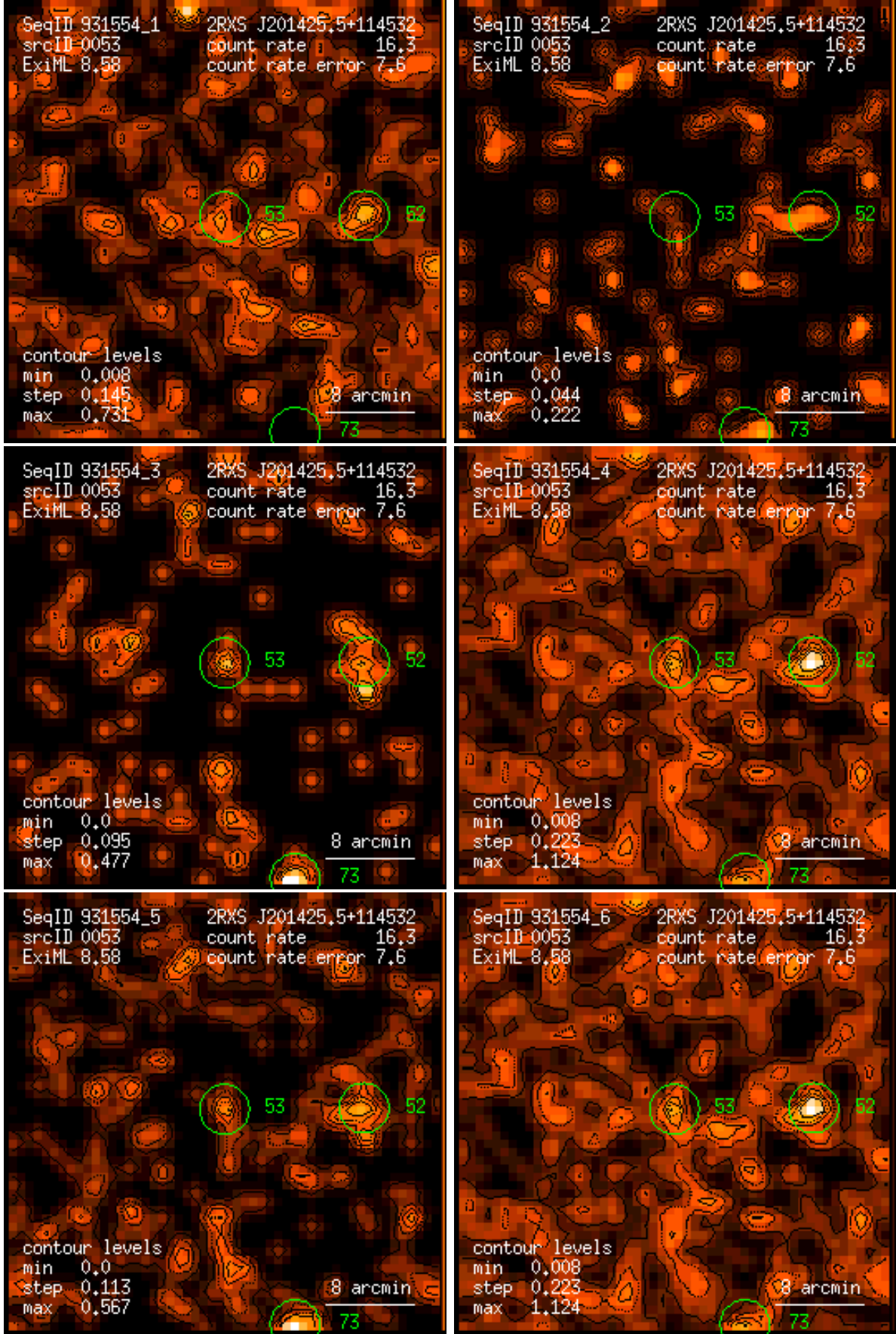
Figure 53: RASS 931554: detection 0053: band rate images, Gaussian filter: (1) PSPC channels 11 – 41, (2) 52 – 90, (3) 91 – 201, (4) 11 – 235, (5) 52 – 201, (6) 11 – 201. Broad band rates in counts/ks. Band rate contour levels in counts/ks/arcmin 2 .
