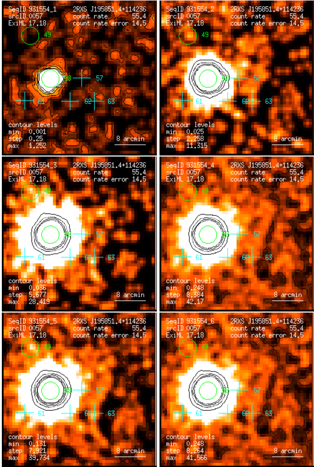
Figure 57: RASS 931554: detection 0057: band rate images, Gaussian filter: (1) PSPC channels 11 – 41, (2) 52 – 90, (3) 91 – 201, (4) 11 – 235, (5) 52 – 201, (6) 11 – 201. Broad band rates in counts/ks. Band rate contour levels in counts/ks/arcmin 2 .
