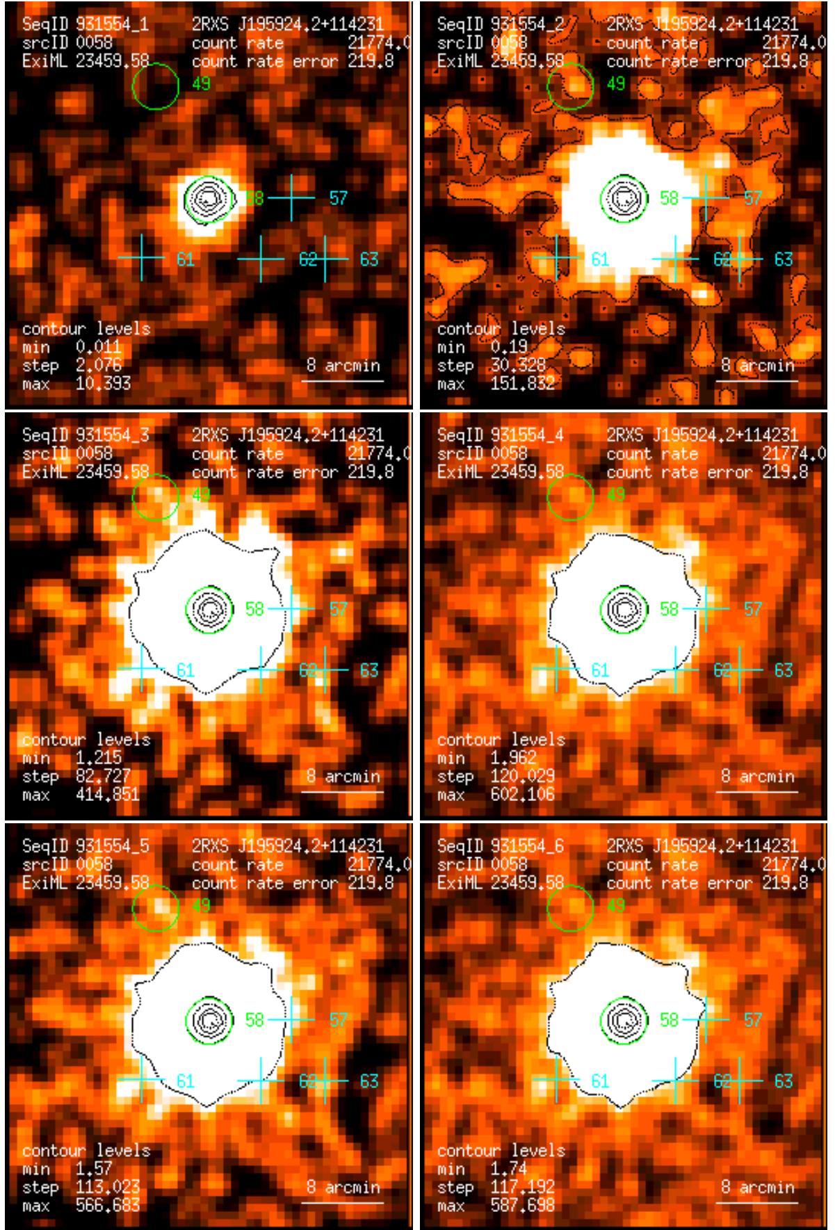
Figure 58: RASS 931554: detection 0058: band rate images, Gaussian filter: (1) PSPC channels 11 – 41, (2) 52 – 90, (3) 91 – 201, (4) 11 – 235, (5) 52 – 201, (6) 11 – 201. Broad band rates in counts/ks. Band rate contour levels in counts/ks/arcmin 2 .
