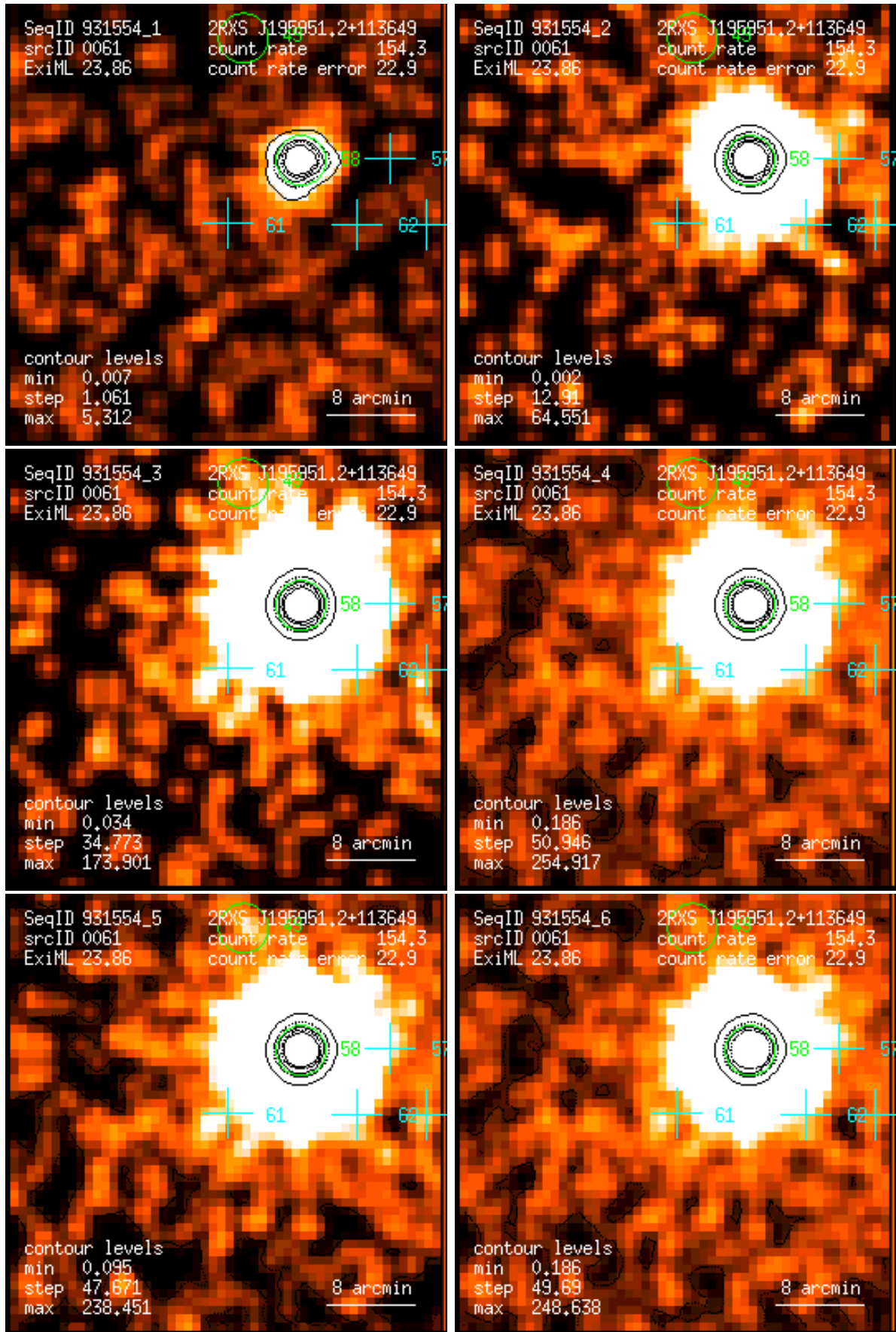
Figure 61: RASS 931554: detection 0061: band rate images, Gaussian filter: (1) PSPC channels 11 – 41, (2) 52 – 90, (3) 91 – 201, (4) 11 – 235, (5) 52 – 201, (6) 11 – 201. Broad band rates in counts/ks. Band rate contour levels in counts/ks/arcmin 2 .
