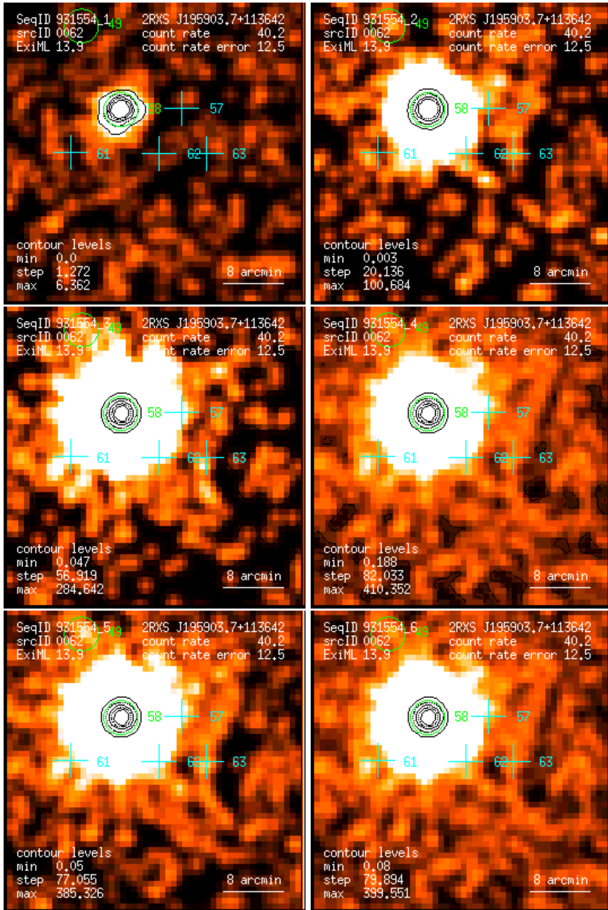
Figure 62: RASS 931554: detection 0062: band rate images, Gaussian filter: (1) PSPC channels 11 – 41, (2) 52 – 90, (3) 91 – 201, (4) 11 – 235, (5) 52 – 201, (6) 11 – 201. Broad band rates in counts/ks. Band rate contour levels in counts/ks/arcmin 2 .
