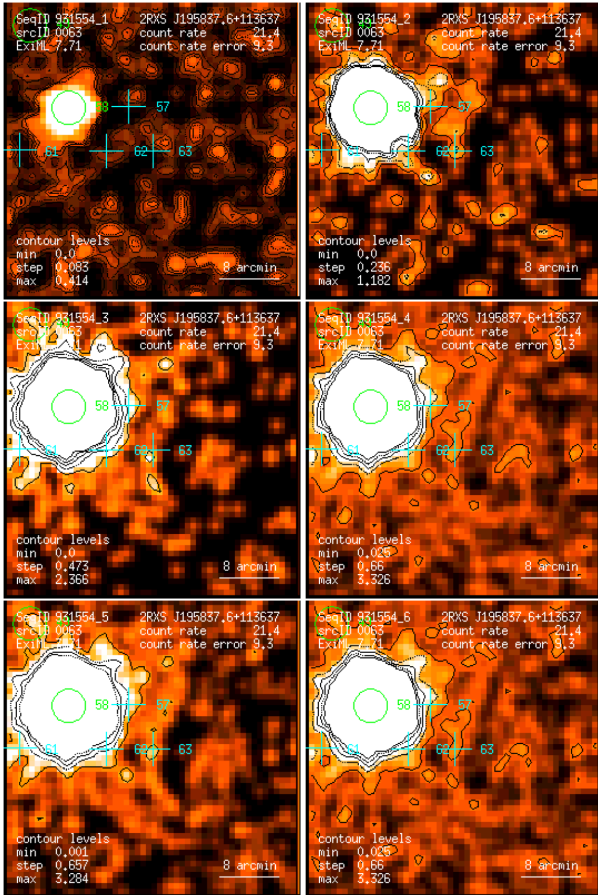
Figure 63: RASS 931554: detection 0063: band rate images, Gaussian filter: (1) PSPC channels 11 – 41, (2) 52 – 90, (3) 91 – 201, (4) 11 – 235, (5) 52 – 201, (6) 11 – 201. Broad band rates in counts/ks. Band rate contour levels in counts/ks/arcmin 2 .
