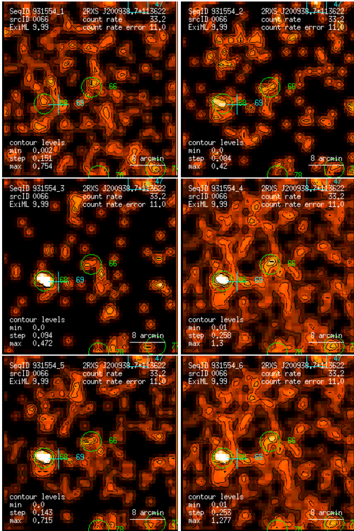
Figure 66: RASS 931554: detection 0066: band rate images, Gaussian filter: (1) PSPC channels 11 – 41, (2) 52 – 90, (3) 91 – 201, (4) 11 – 235, (5) 52 – 201, (6) 11 – 201. Broad band rates in counts/ks. Band rate contour levels in counts/ks/arcmin 2 .
