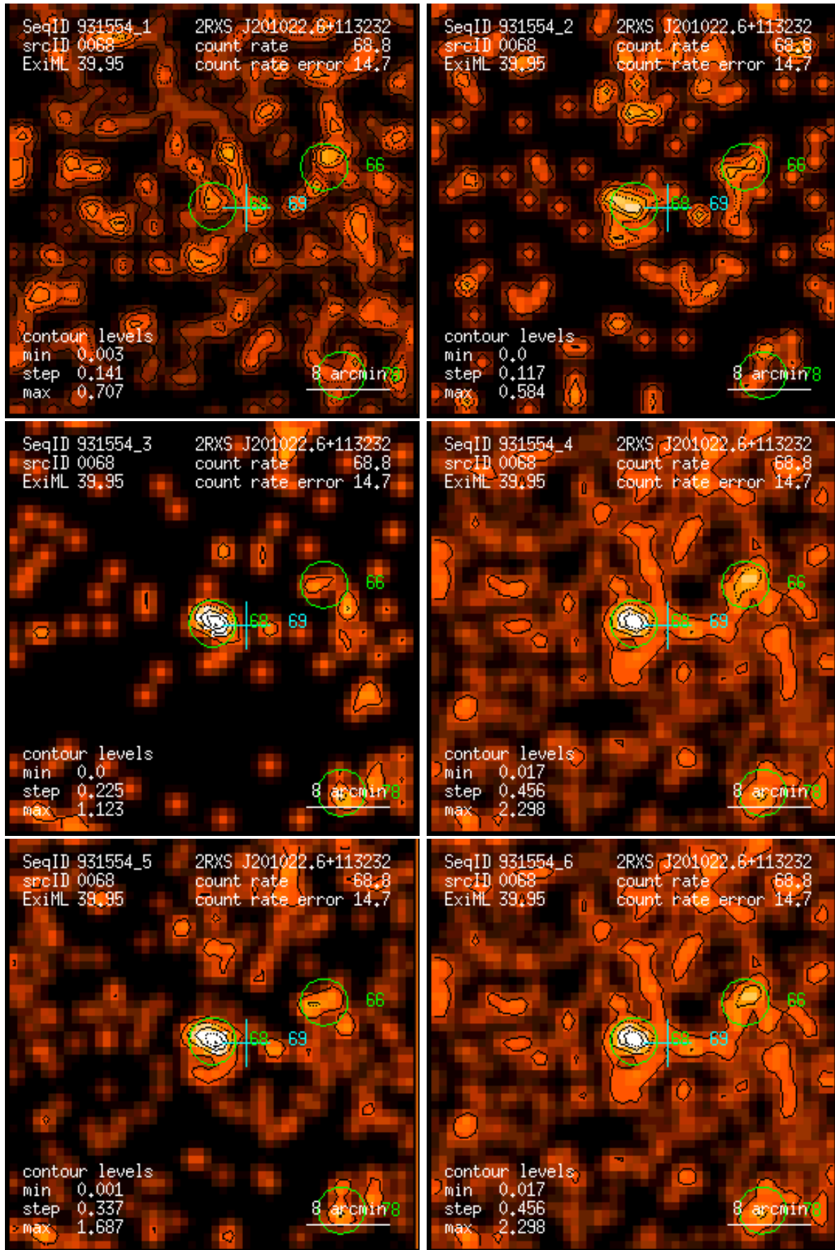
Figure 68: RASS 931554: detection 0068: band rate images, Gaussian filter: (1) PSPC channels 11 – 41, (2) 52 – 90, (3) 91 – 201, (4) 11 – 235, (5) 52 – 201, (6) 11 – 201. Broad band rates in counts/ks. Band rate contour levels in counts/ks/arcmin 2 .
