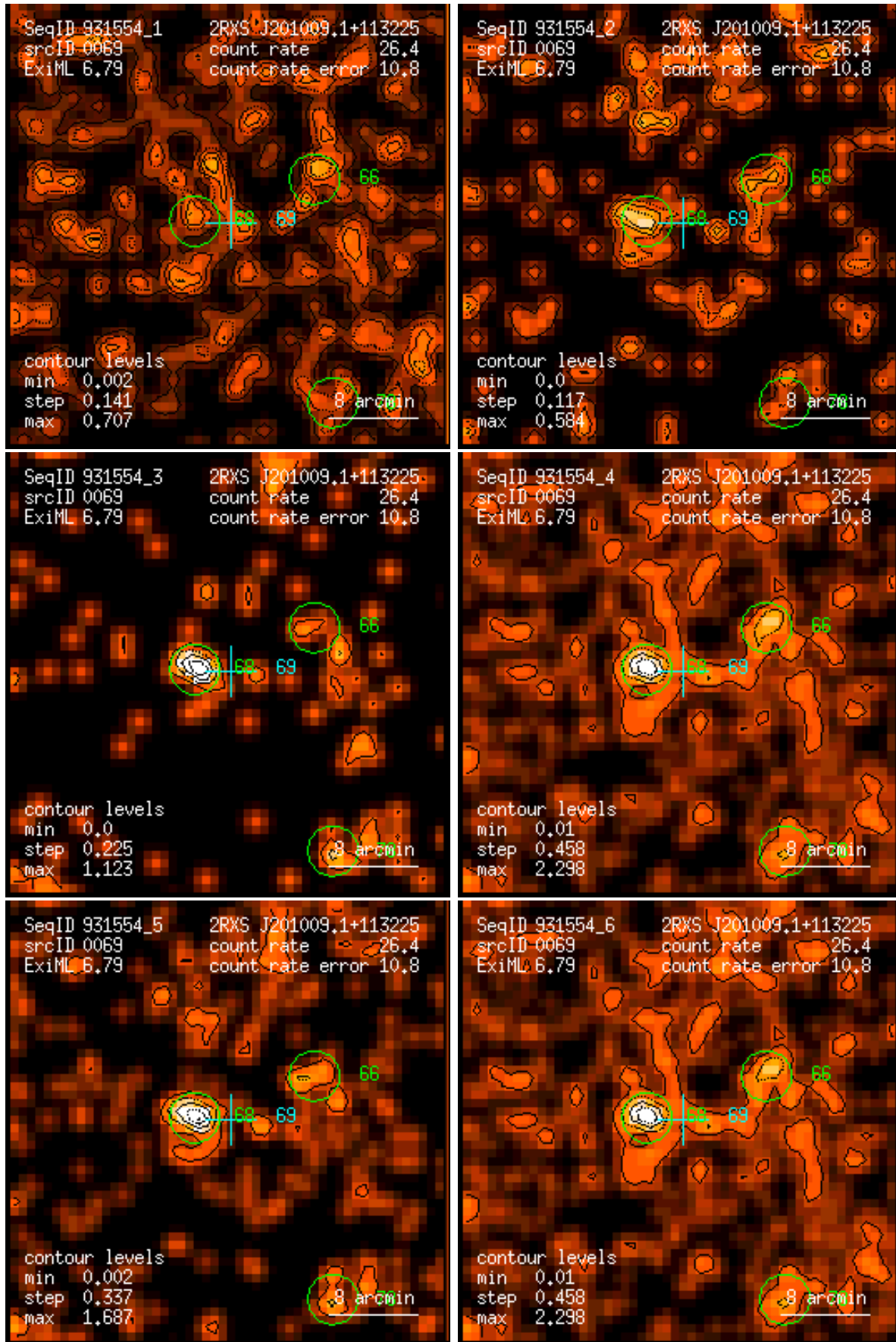
Figure 69: RASS 931554: detection 0069: band rate images, Gaussian filter: (1) PSPC channels 11 – 41, (2) 52 – 90, (3) 91 – 201, (4) 11 – 235, (5) 52 – 201, (6) 11 – 201. Broad band rates in counts/ks. Band rate contour levels in counts/ks/arcmin 2 .
