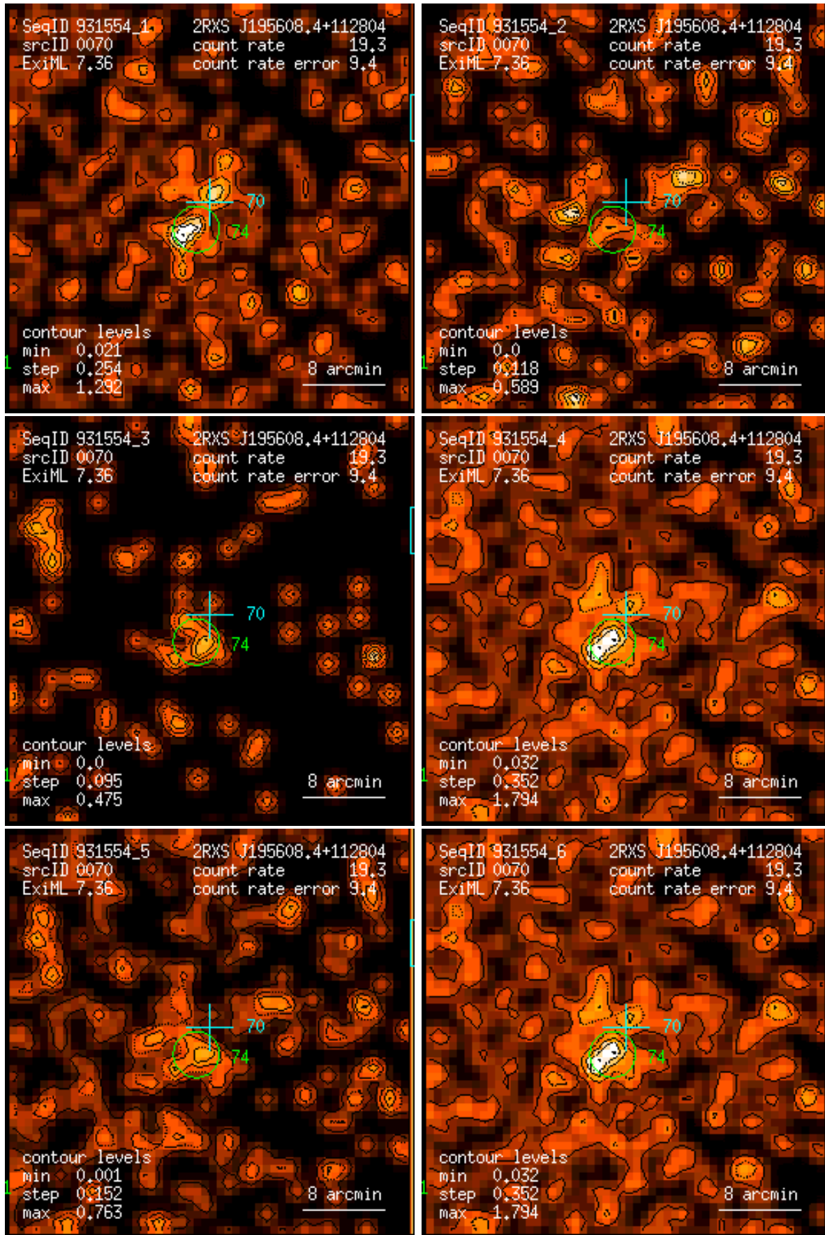
Figure 70: RASS 931554: detection 0070: band rate images, Gaussian filter: (1) PSPC channels 11 – 41, (2) 52 – 90, (3) 91 – 201, (4) 11 – 235, (5) 52 – 201, (6) 11 – 201. Broad band rates in counts/ks. Band rate contour levels in counts/ks/arcmin 2 .
