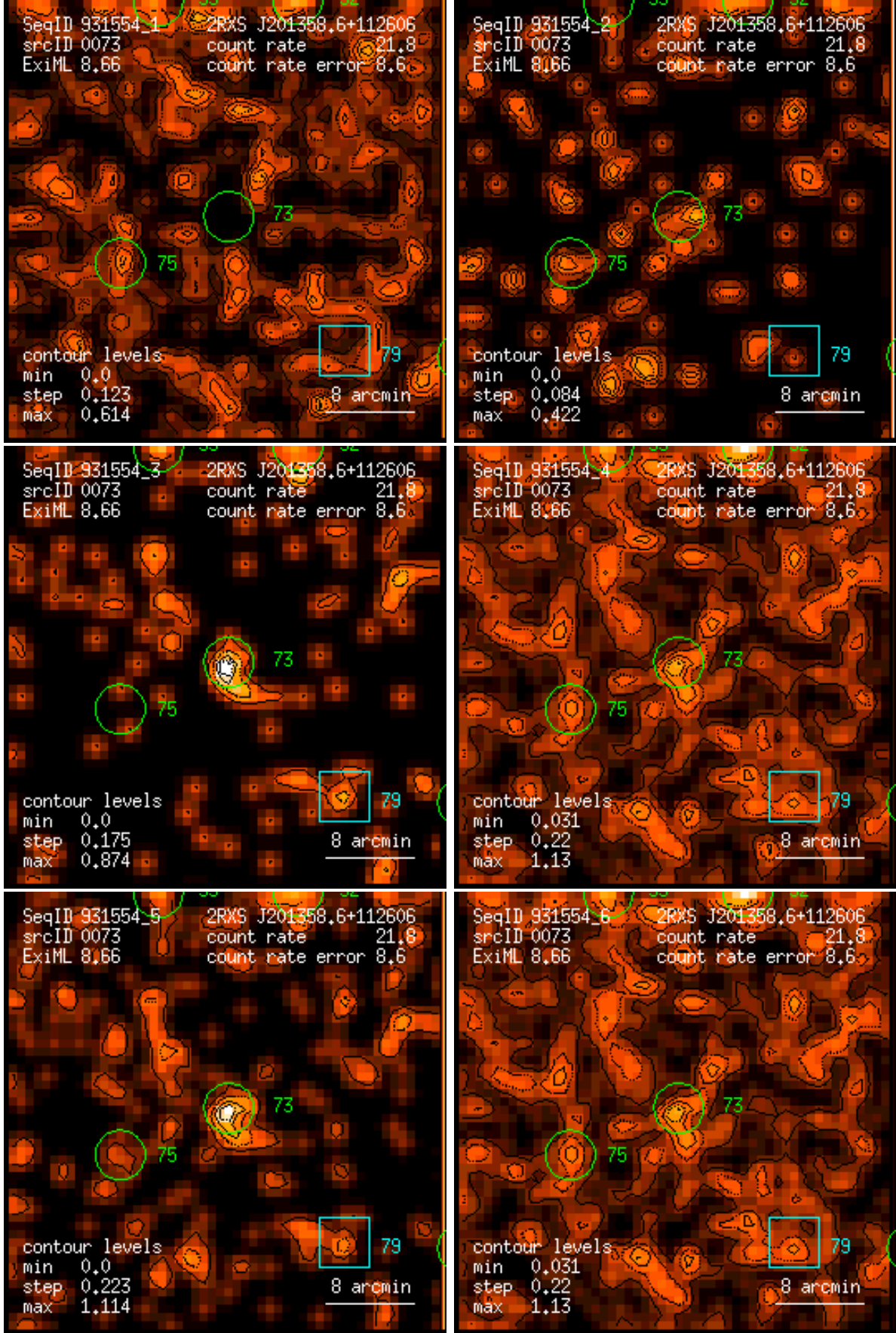
Figure 73: RASS 931554: detection 0073: band rate images, Gaussian filter: (1) PSPC channels 11 – 41, (2) 52 – 90, (3) 91 – 201, (4) 11 – 235, (5) 52 – 201, (6) 11 – 201. Broad band rates in counts/ks. Band rate contour levels in counts/ks/arcmin 2 .
