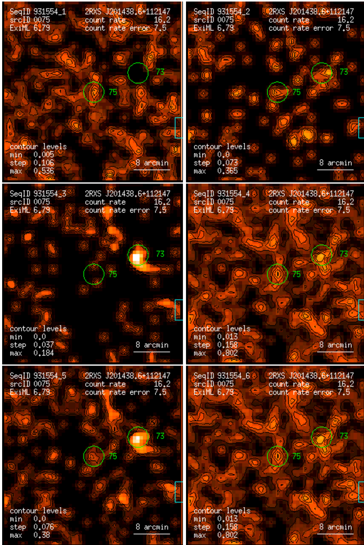
Figure 75: RASS 931554: detection 0075: band rate images, Gaussian filter: (1) PSPC channels 11 – 41, (2) 52 – 90, (3) 91 – 201, (4) 11 – 235, (5) 52 – 201, (6) 11 – 201. Broad band rates in counts/ks. Band rate contour levels in counts/ks/arcmin 2 .
