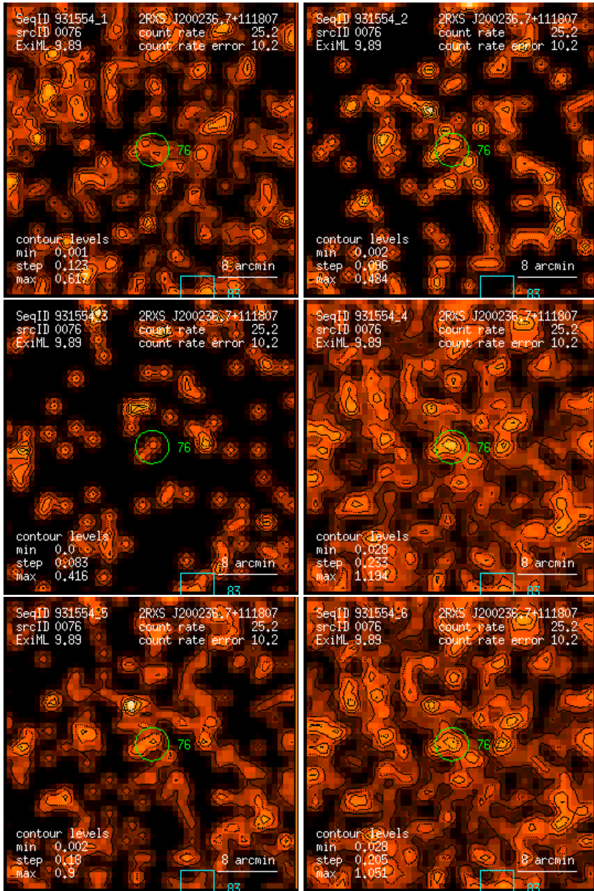
Figure 76: RASS 931554: detection 0076: band rate images, Gaussian filter: (1) PSPC channels 11 – 41, (2) 52 – 90, (3) 91 – 201, (4) 11 – 235, (5) 52 – 201, (6) 11 – 201. Broad band rates in counts/ks. Band rate contour levels in counts/ks/arcmin 2 .
