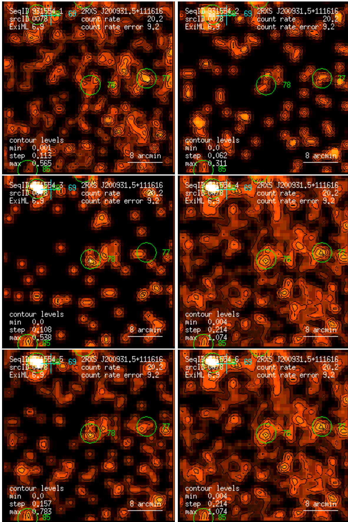
Figure 78: RASS 931554: detection 0078: band rate images, Gaussian filter: (1) PSPC channels 11 – 41, (2) 52 – 90, (3) 91 – 201, (4) 11 – 235, (5) 52 – 201, (6) 11 – 201. Broad band rates in counts/ks. Band rate contour levels in counts/ks/arcmin 2 .
